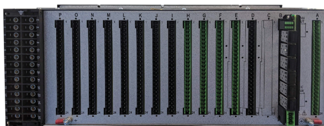
Figure 4 DS Agile C264 rear view (80TE case)
