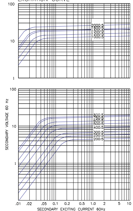
EXCITATION CURVE
