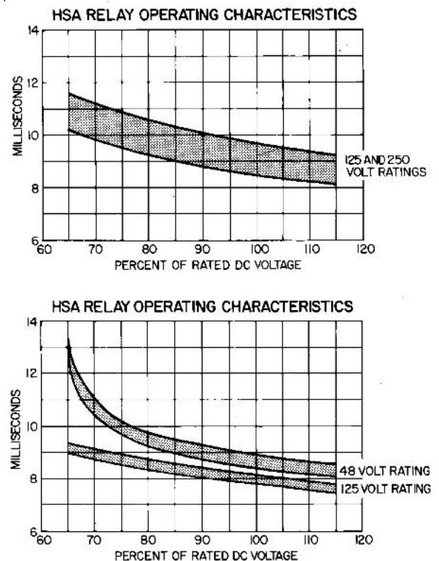
Fig. 3. Operating characteristics, 8- and 11-stage HSA relays
