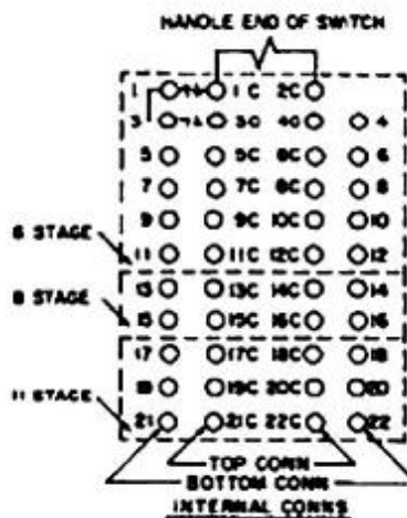
Fig. 2. HSA11 Relay Contacts
