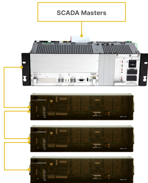
Figure 1: Simple architecture of I/O modules communicating to the D20 RTU
