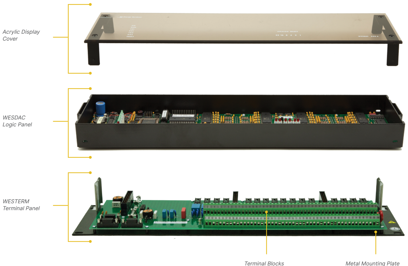
Figure 2: Architecture of I/O logic and termination panels
