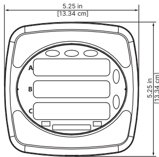
P40NPLUS Front Dimensions
