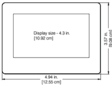
P70N Front Dimensions
