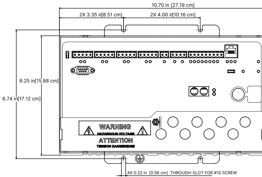
EPM 9700 Front Dimensions
