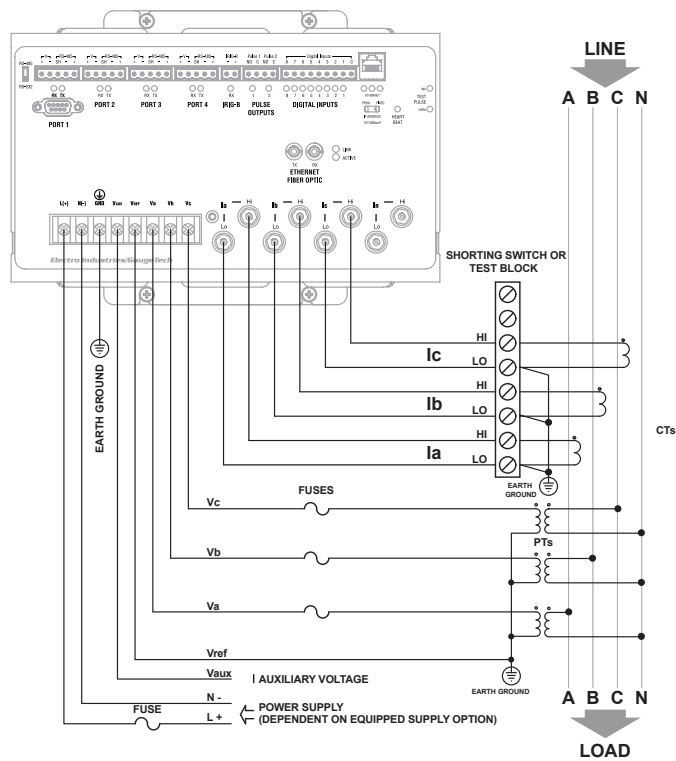
4-Wire Wye, 3-Element with 3 PTs and 3 CTs
