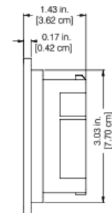
P70N Side Dimensions
