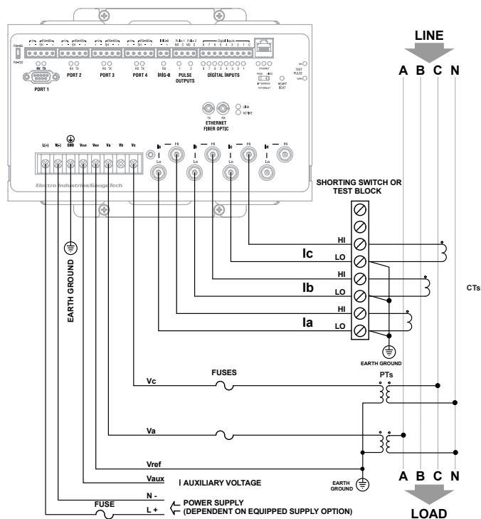
3 Phase, 4 Wire 2.5-Element with 2 PTs, 3 CTs
