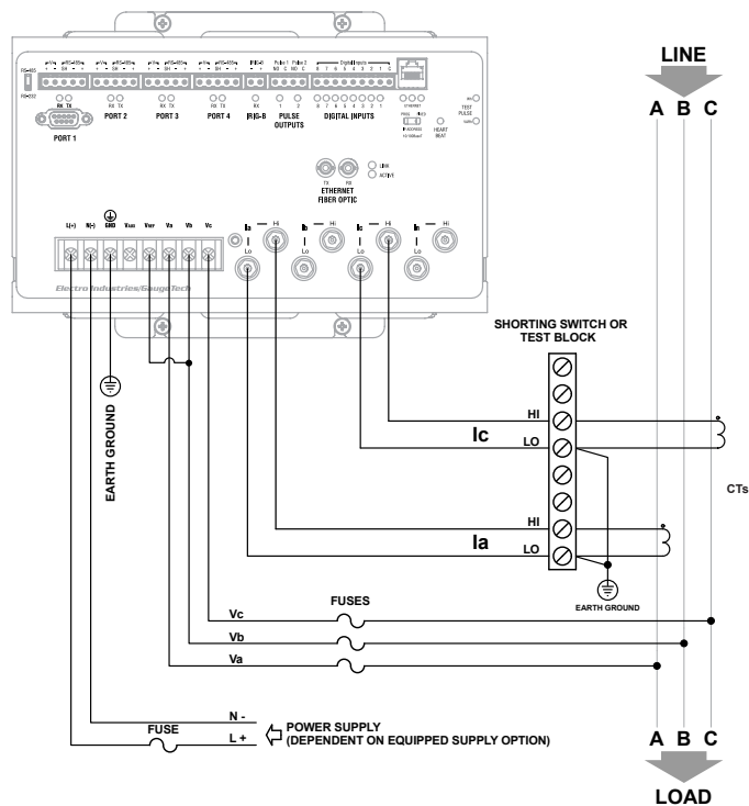
3 Wire, 2 Element Delta Direct Voltage with 2 CTs Important: The Potential between A, B, C and GROUND must be less than 347 V AC
