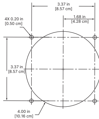
P40NPLUS Back Dimensions
