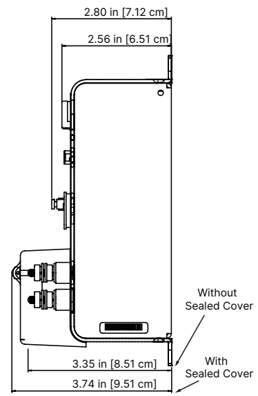
EPM 9700 Side Dimensions
