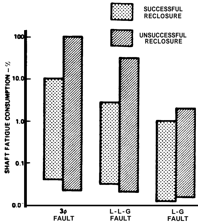
Fig. 5. Ranges of shaft fatigue duty (single incident)
