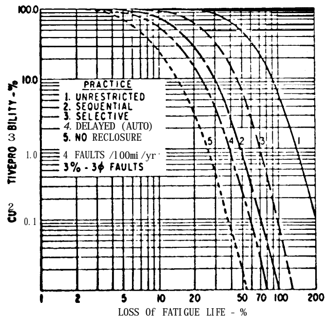
Fig. 8. Fatigue expenditure over 40-year exposure period (3 percent 3 \phi faults)
