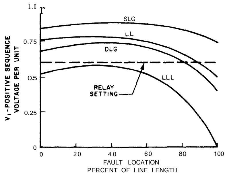
(8) VOLTAGES AS SEEN AT THE RECEIVING END. (80-MILE LINE)
