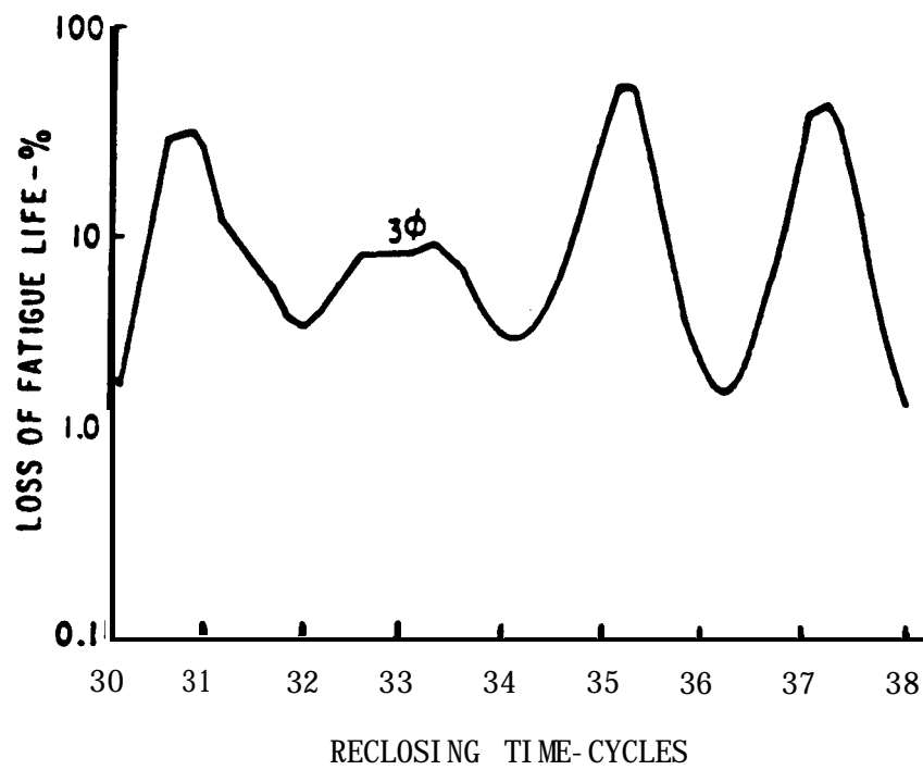
Fig. 6. Effect of breaker reclosing time on shaft fatigue duty
