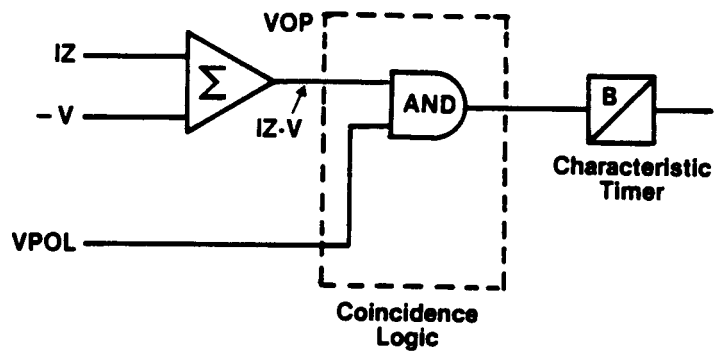
a. Simple Phase Angle Comparer
