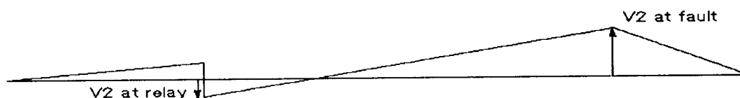
c. Negative Sequence Voltage Profile (capacitor gaps not flashed),
