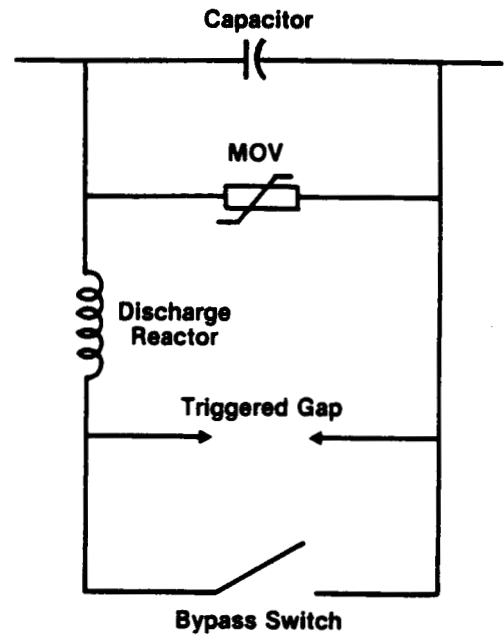
Metal Oxide Varistor
