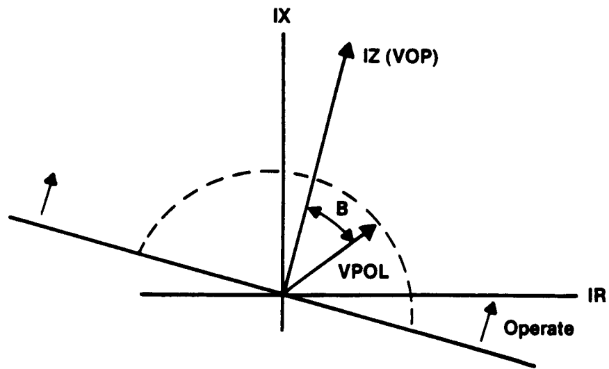
Phasor Diagram for Simple Directional Function
