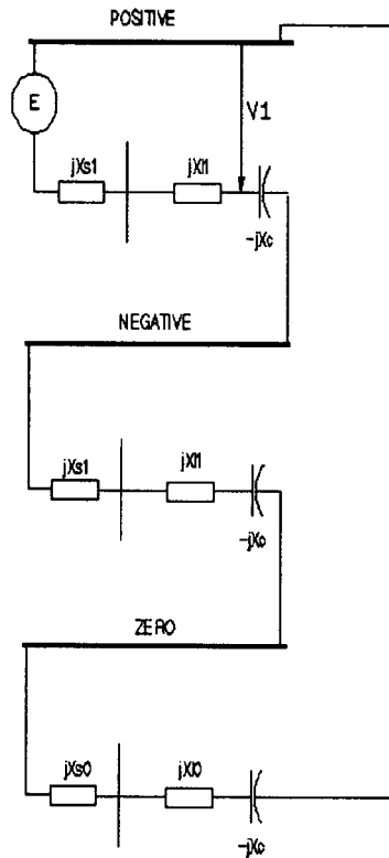
b. Network Connections for Phase-to-Ground Fault
