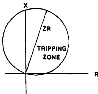
R-X IMPEDANCE DIAGRAM
