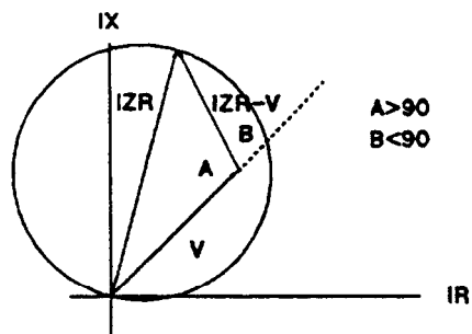
INTERNAL FAULT
