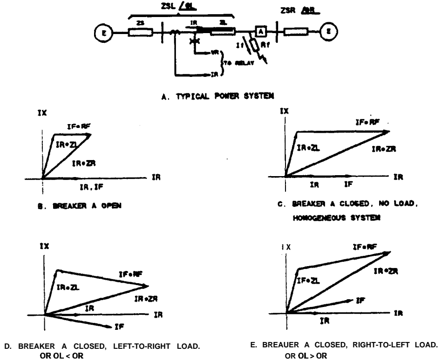
Figure 24 - Effect of load flow and system non-homogeneity on fault resistance
