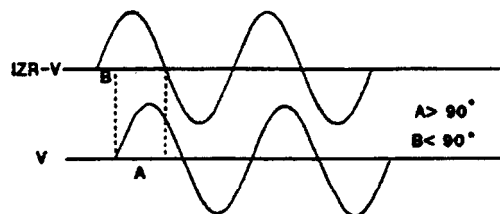
INTERNAL FAULT RR-V LEADS V BY LESS THAN 90 DEGREES
