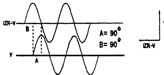
MHO CHARACTERISTIC BALANCE POINT
