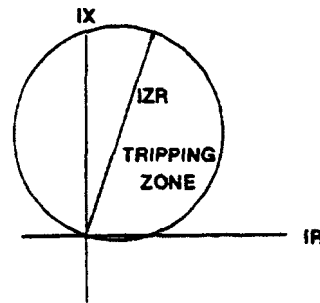
IR-IX VOLTAGE DIAGRAM
