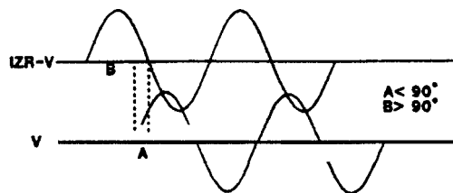
EXTERNAL FAULT IZR-V LEADS V BY MORE THAN 90 DEGREES
