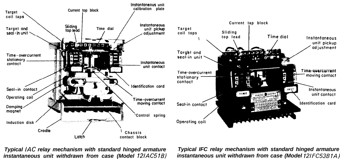
Fig. 1. Typical IAC and IFC time-overcurrentrelays
