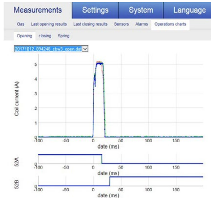
Coil Current - Opening
