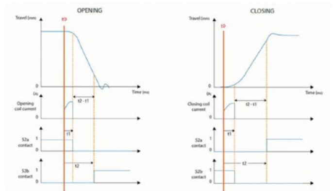
Operation timing point charts
