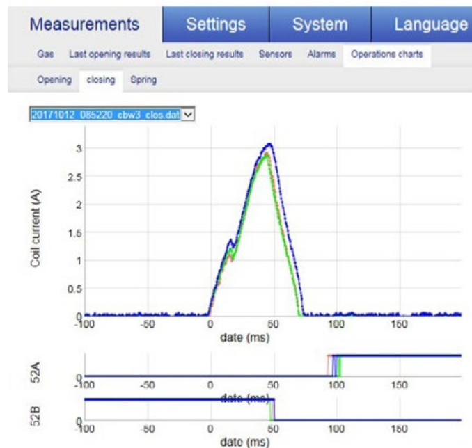
Coil Current - Closing
