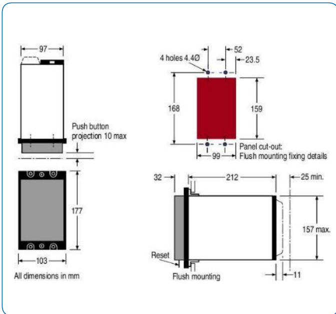
Figure 2 MVTP 11. Case outline size 4
