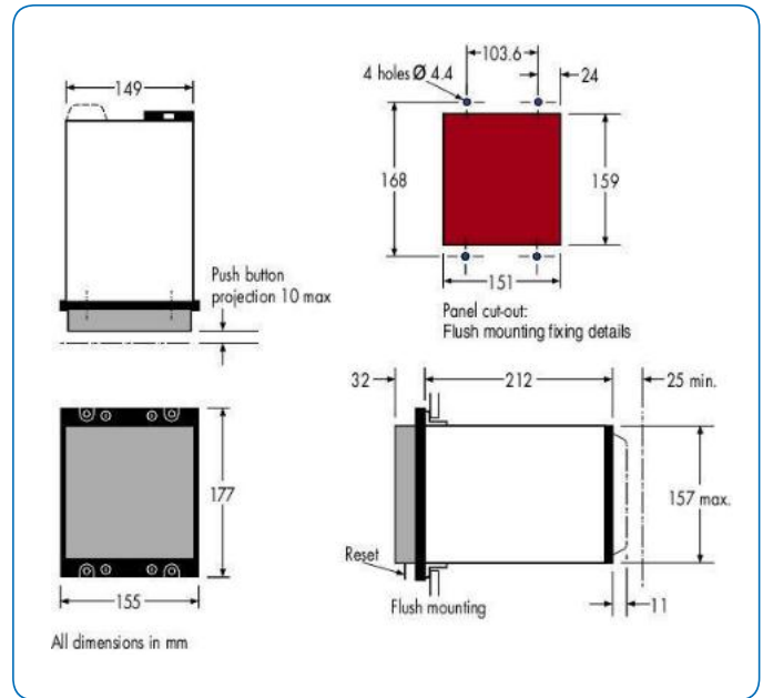
Figure 3 MVTP 31. Case outline size 6
