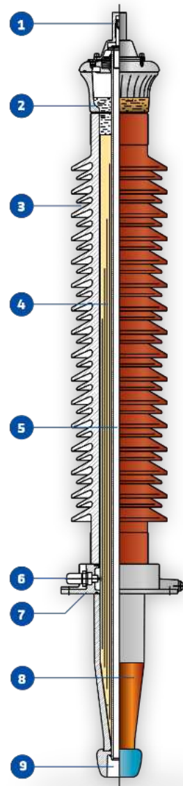
Fig. 1: Bushings 36 to 170 kV Normal Cantilever load
