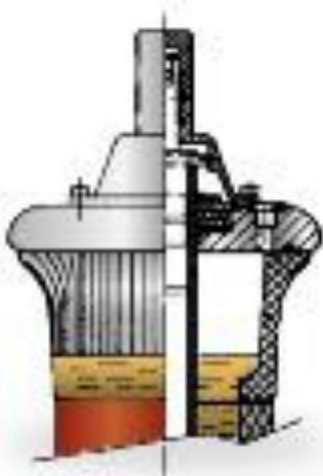
Fig. 2: Oil level indicator for prismatic glass and metal head
