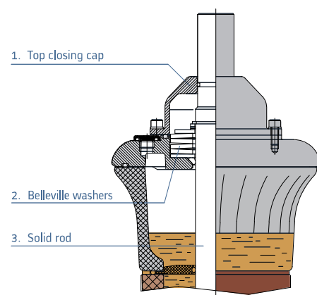
Fig. 7: H2 head type (Bottom connection)
