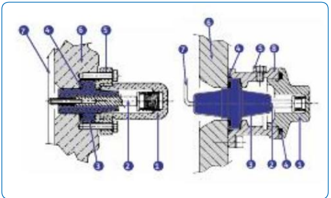
Fig. 3: Power Factor Tap
