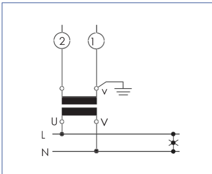
Volts, frequency
