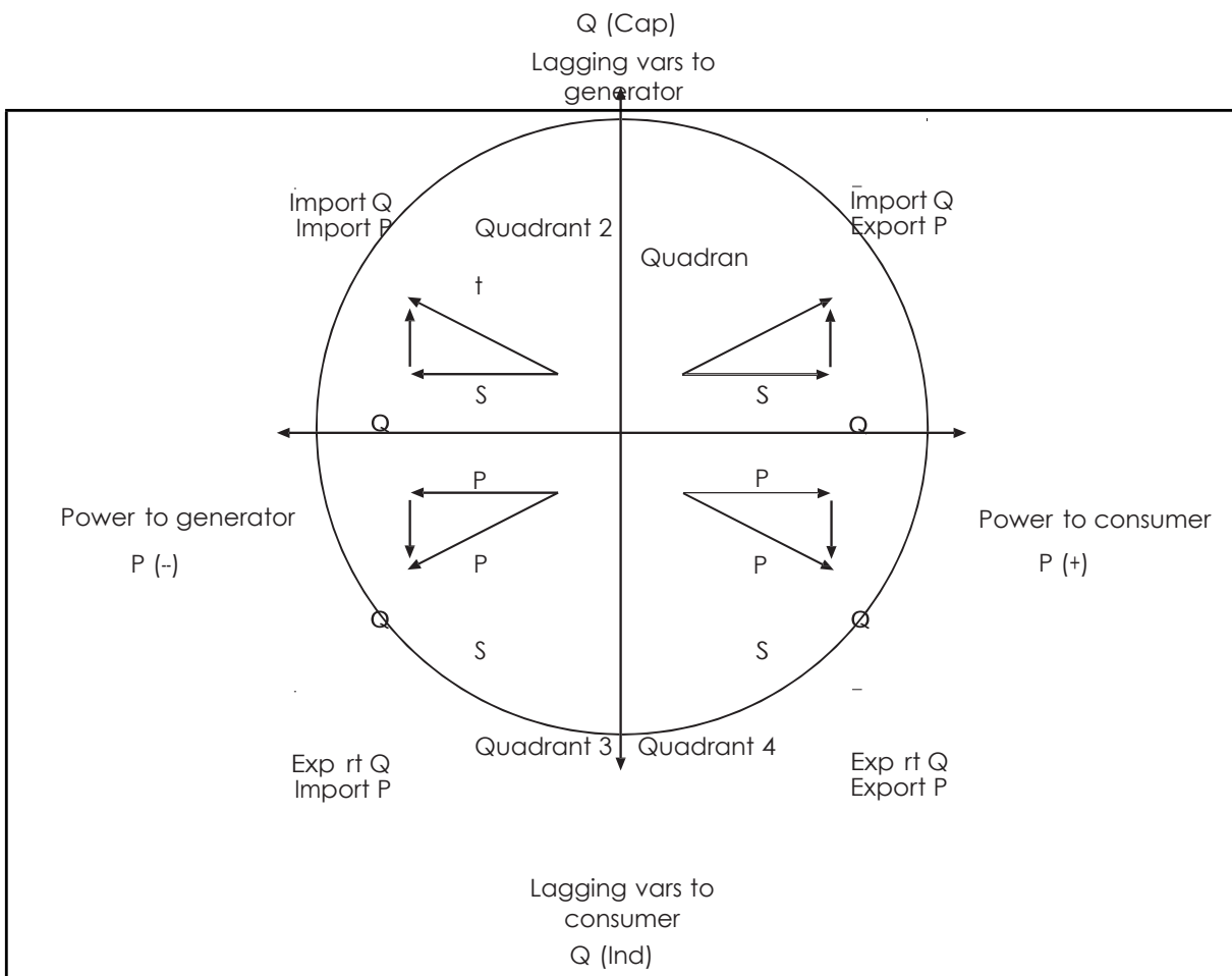
FIGURE 4-1: POWER FLOW
