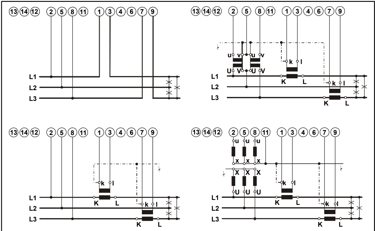
FIGURE 10-5: EXTERNAL WIRING DIAGRAM: 3-PHASE, 3-WIRE UNBALANCED LOAD (3U)
