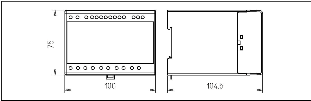
FIGURE 10-8: ENCLOSURE DIMENSIONS
