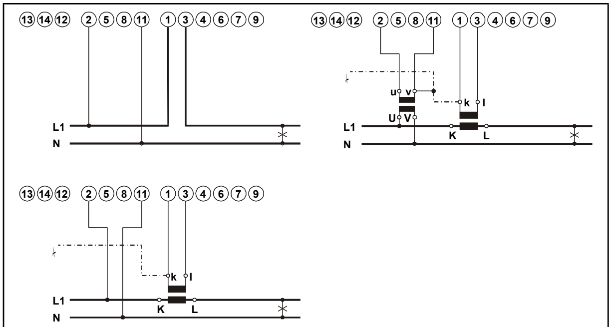
FIGURE 10-2: EXTERNAL WIRING DIAGRAM: SINGLE PHASE (1B)
