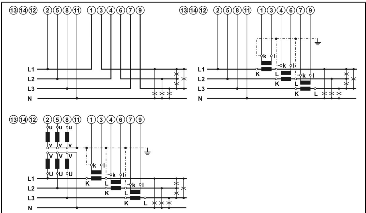
FIGURE 10-6: EXTERNAL WIRING DIAGRAM: 3-PHASE, 4-WIRE UNBALANCED LOAD (4U)
