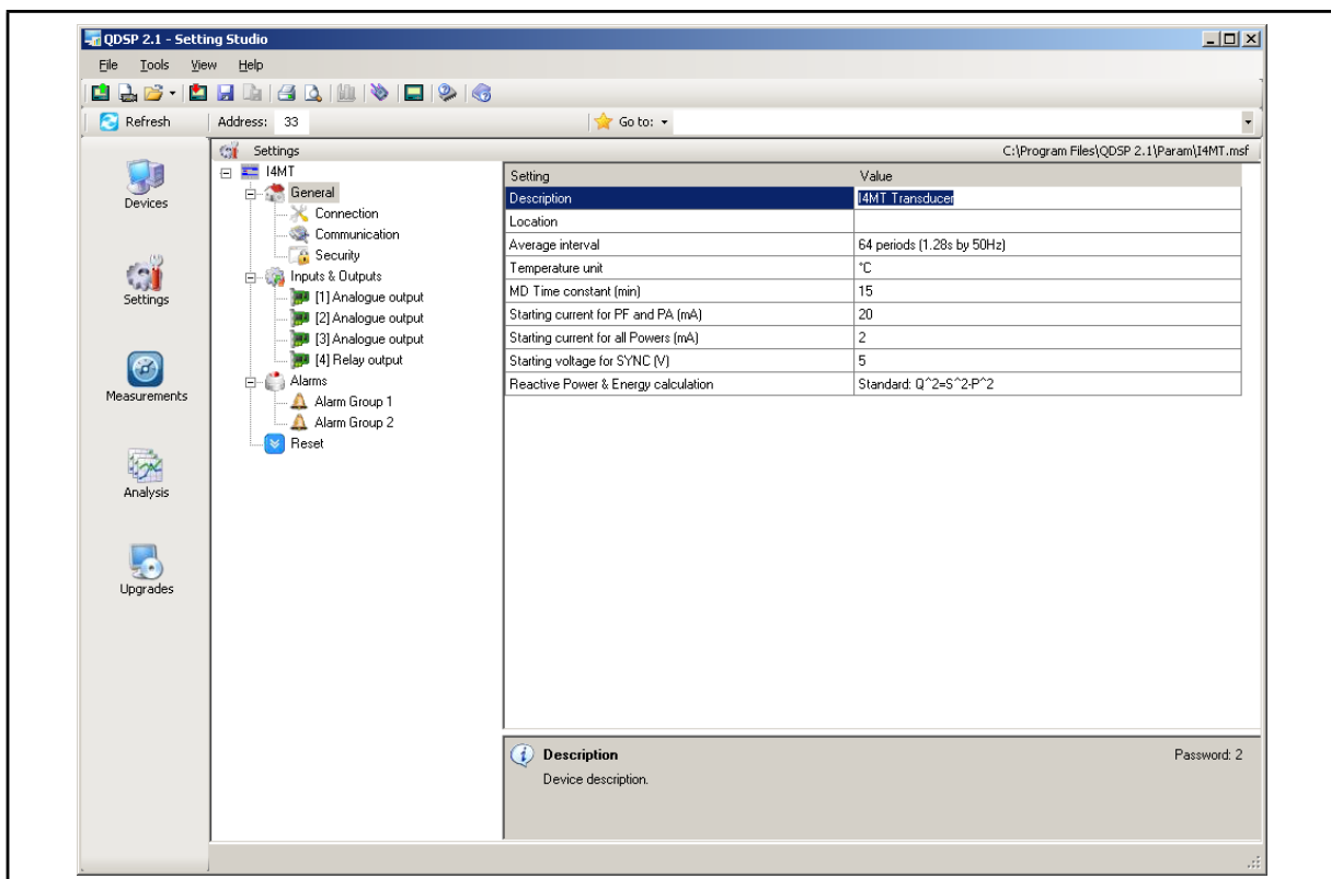
FIGURE 3-1: QDSP INTERFACE
