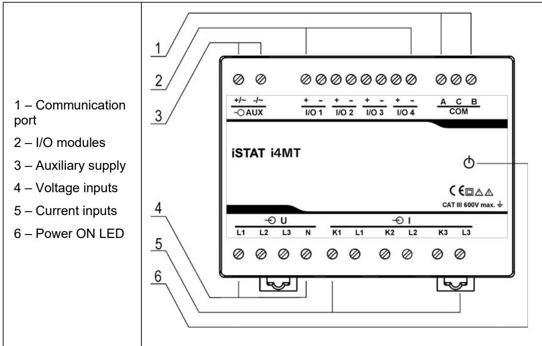
FIGURE 2-1: I4MT SHOWING CONNECTIONS
