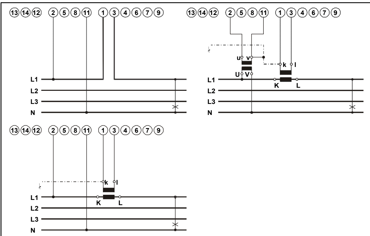
FIGURE 10-4: EXTERNAL WIRING DIAGRAM: 3-PHASE, 4-WIRE BALANCED LOAD (4B)
