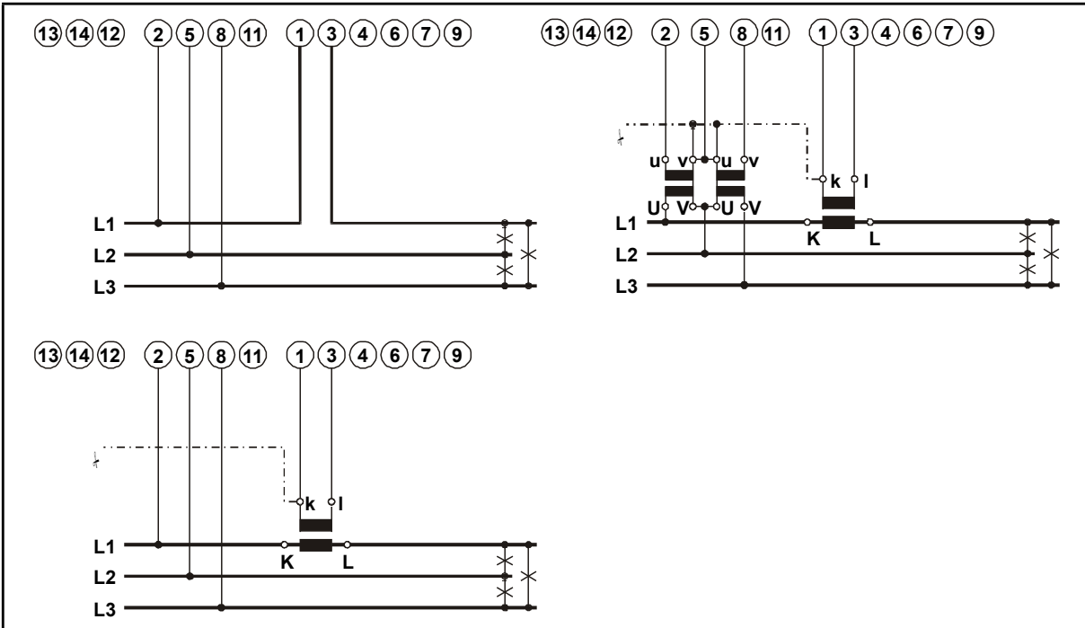
FIGURE 10-3: EXTERNAL WIRING DIAGRAM: 3-PHASE, 3-WIRE BALANCED LOAD (3B)
