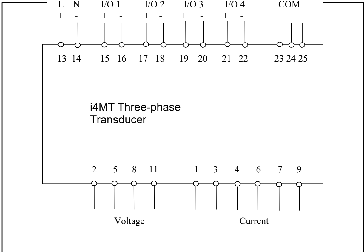
FIGURE 10-1: CONNECTION DIAGRAM
