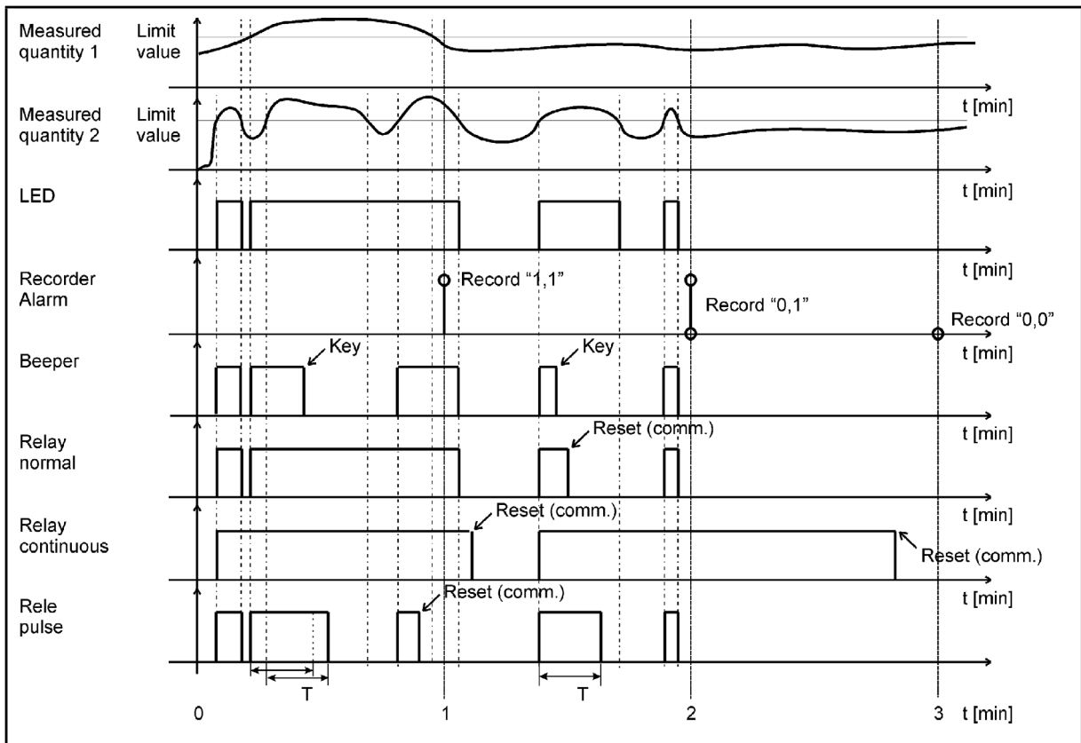
FIGURE 9-9 : ALARM OUTPUTS
