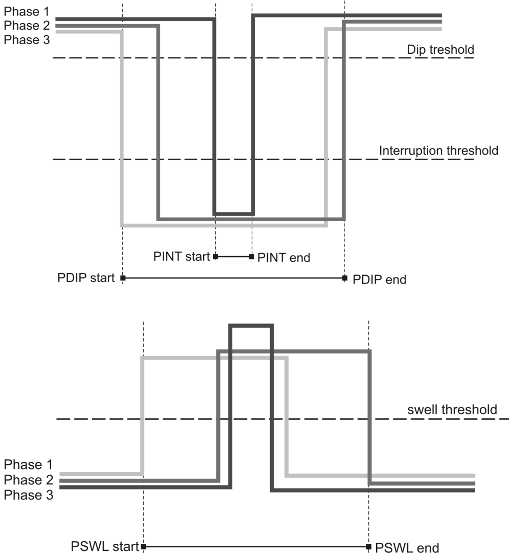
Graphical presentation of multiphase (PDIP, PINT, PSWL) event detection
