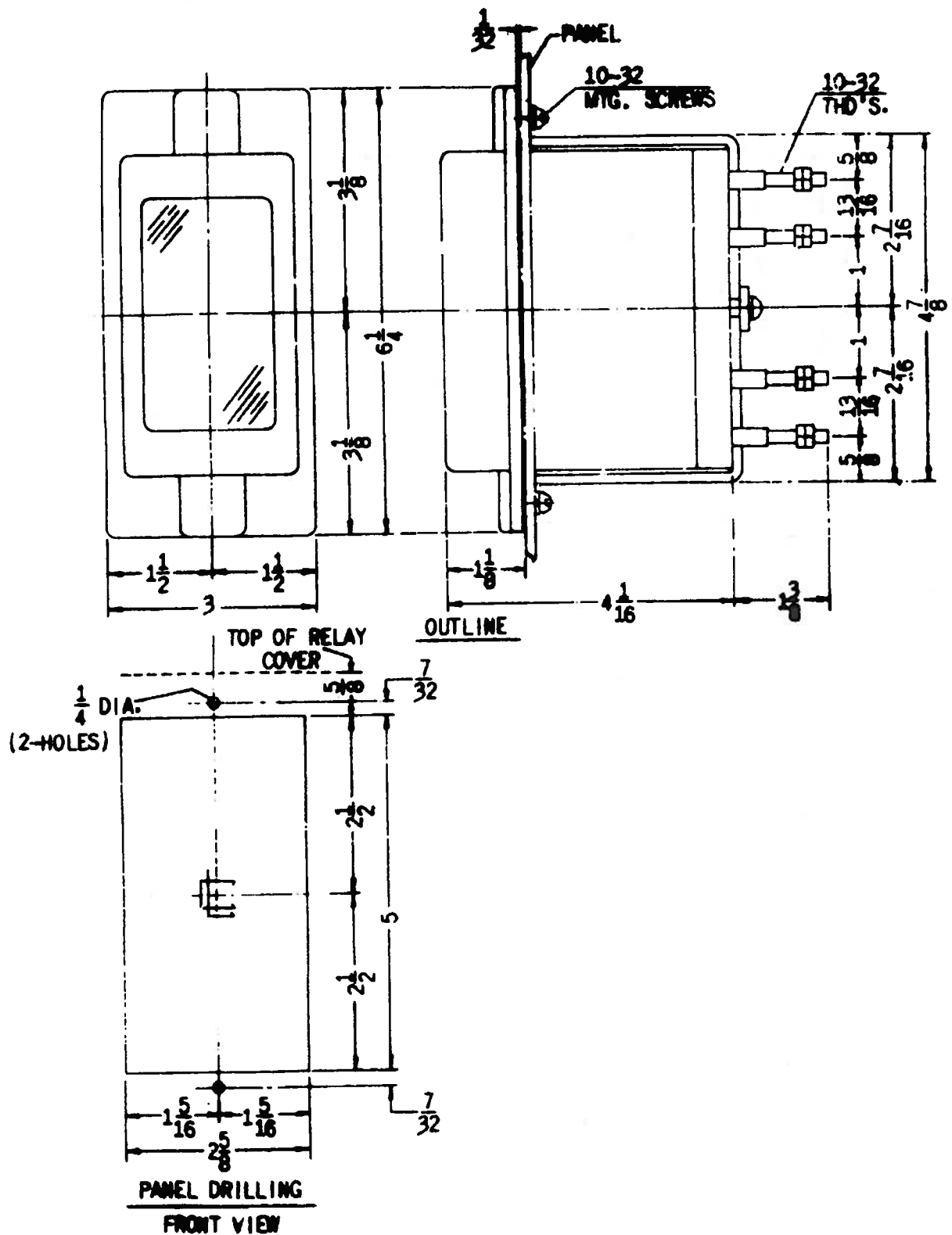
Fig. 3 (104A8558-2) Outline and Panel Drilling for Flush Mounted Back Connected HGA14D Relay.
