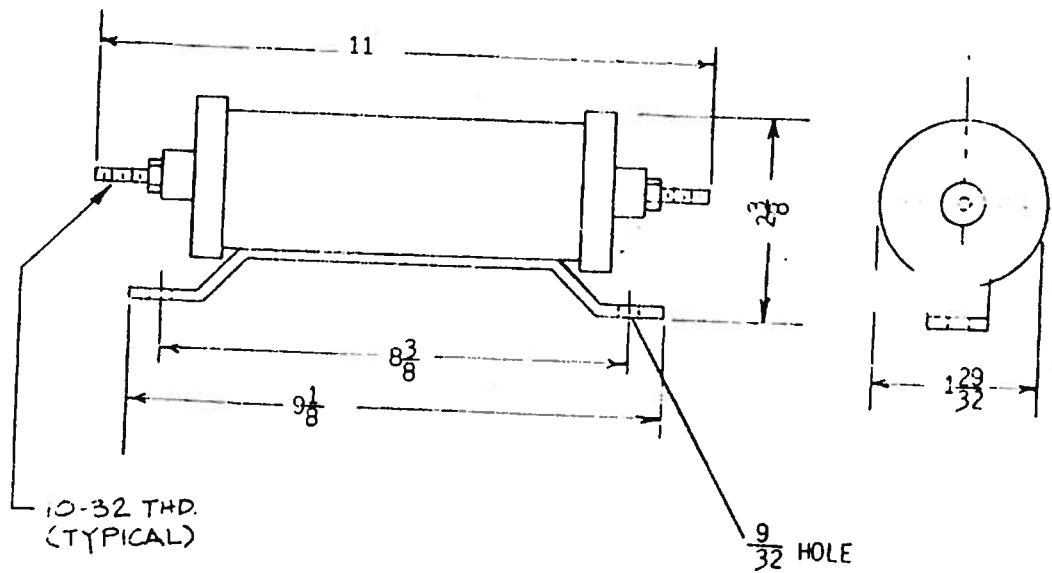
* Fig. 4 Outline of External Resistor used with Forms 25 and 26 of these Relays
