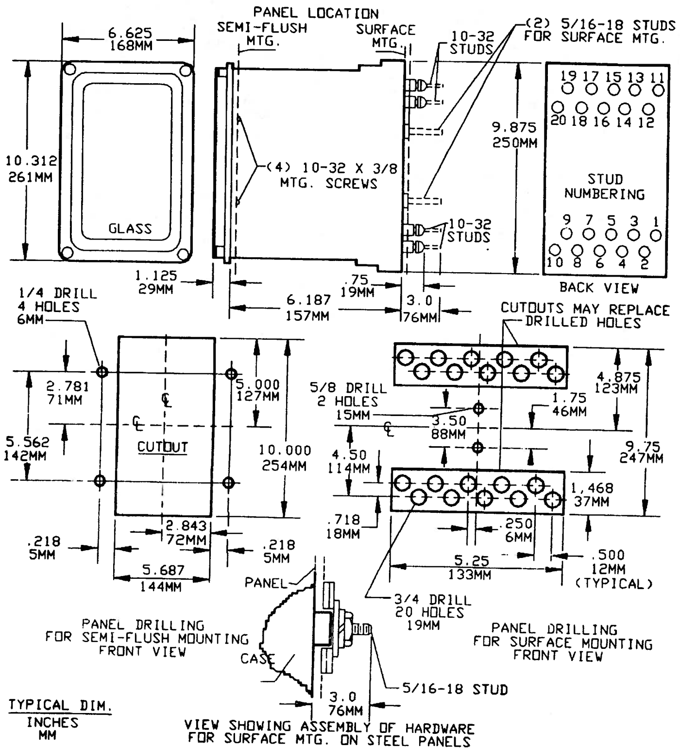
Figure 3 (K-6209272 [8]) Outline and Panel Drilling Dimensions for Type HGA11N Relay
