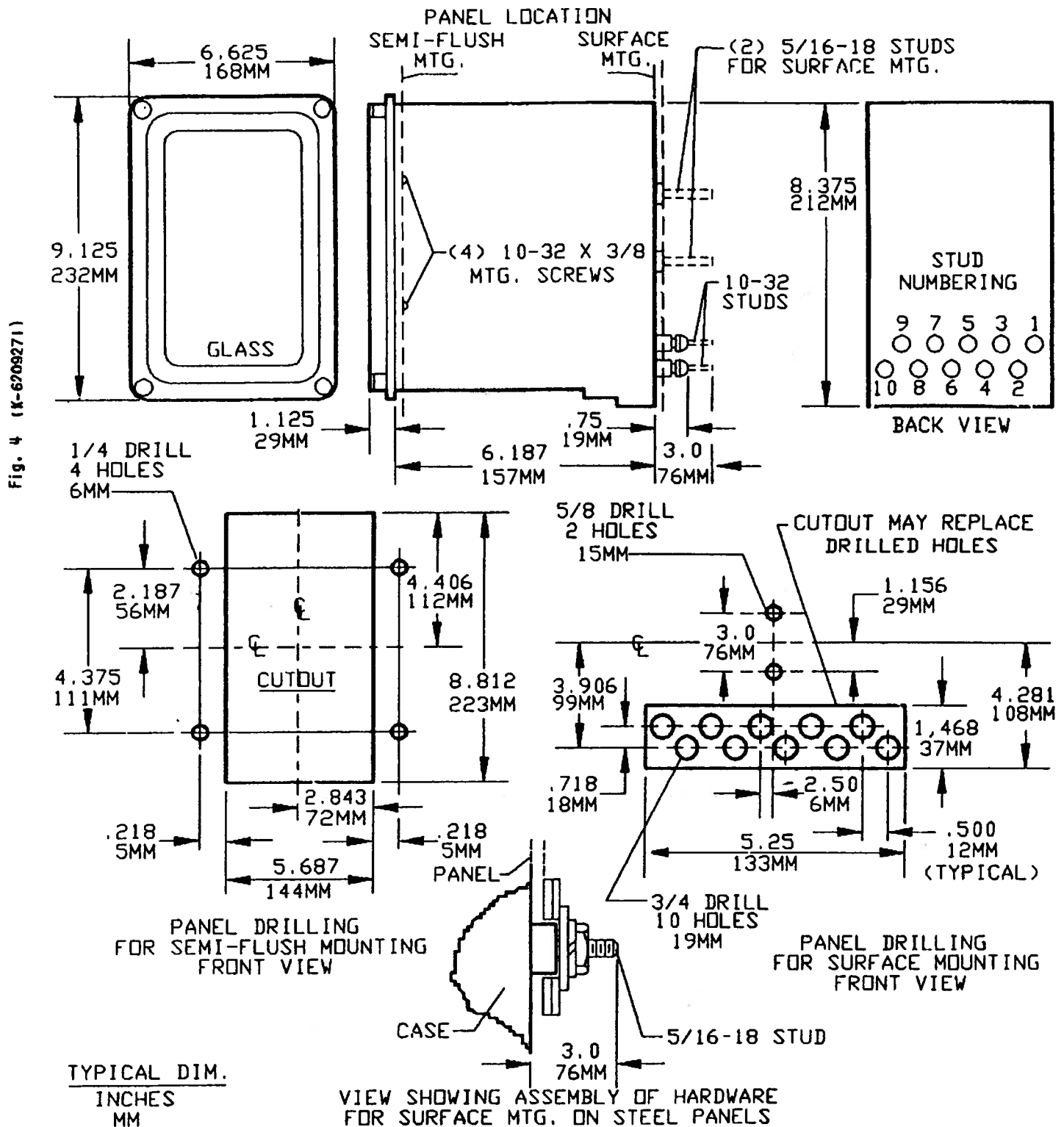
Figure 4 (K-6209271 [8]) Outline And Panel Drilling Dimensions For Type HGA11R Relay
