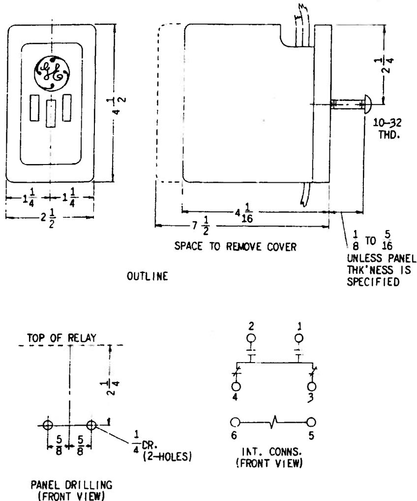
Fig. 1 Outline, Panel Drilling and Internal Connection Diagram for the HGA26C Relay
