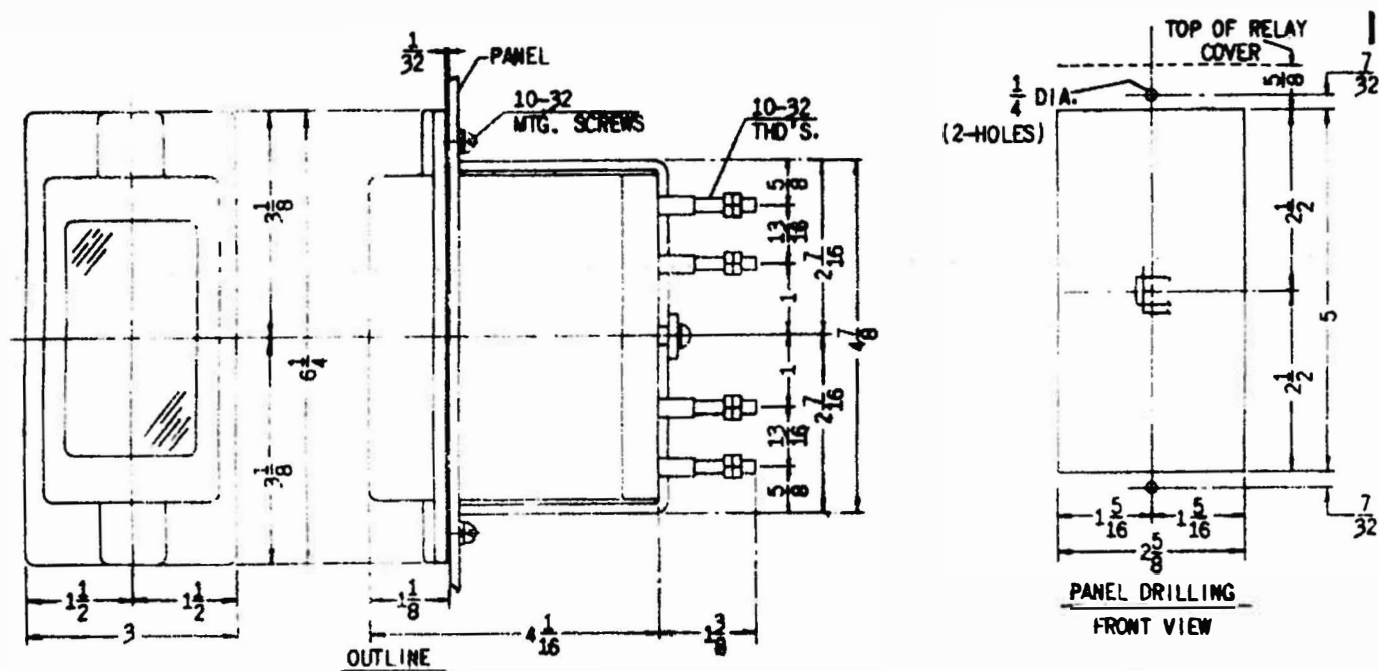
Fig. 6 Outline and Panel Drilling Diagram for HGA1488 Relay (Semi-flush Mounted)
