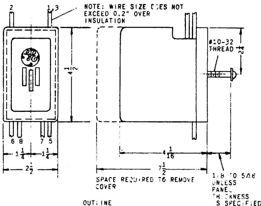
Fig. 4 Outline and Panel Drilling Diagram for HGA14BA Relay (Surface Mounted)
