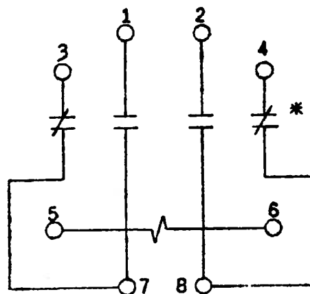
INTERNAL CONNECTIONS (BACK VIEW)
