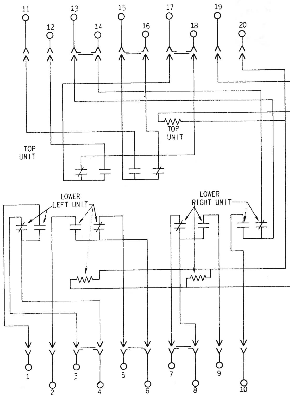
FIG. 1 (0226A6955-0) Internal Connections Diagram For The HGA11E Relay (Front View)
