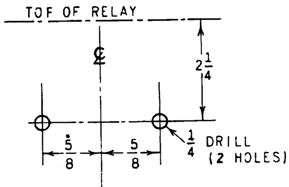
PANEL DRILLING (FRONT VIEW)
