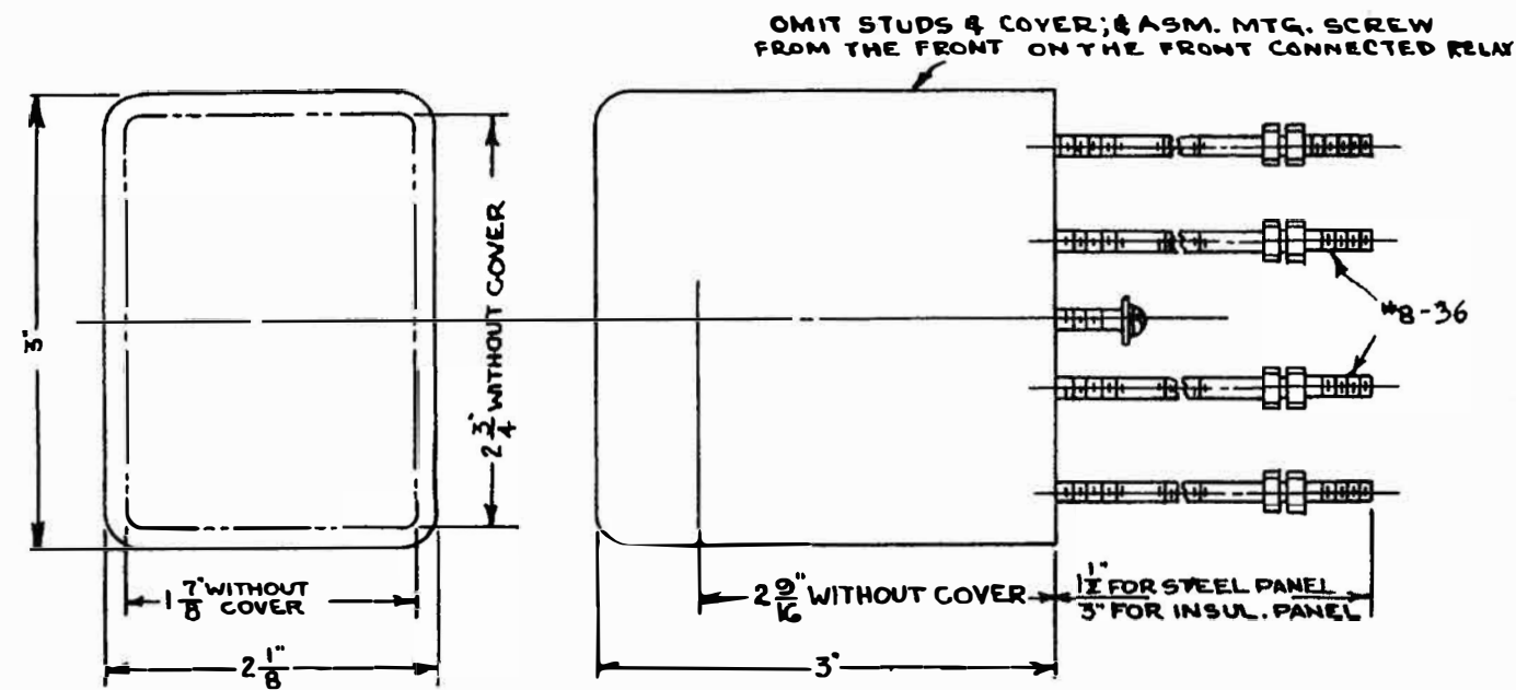
OUTLINE (FRONT & BACK CONNECTED RELAY)
