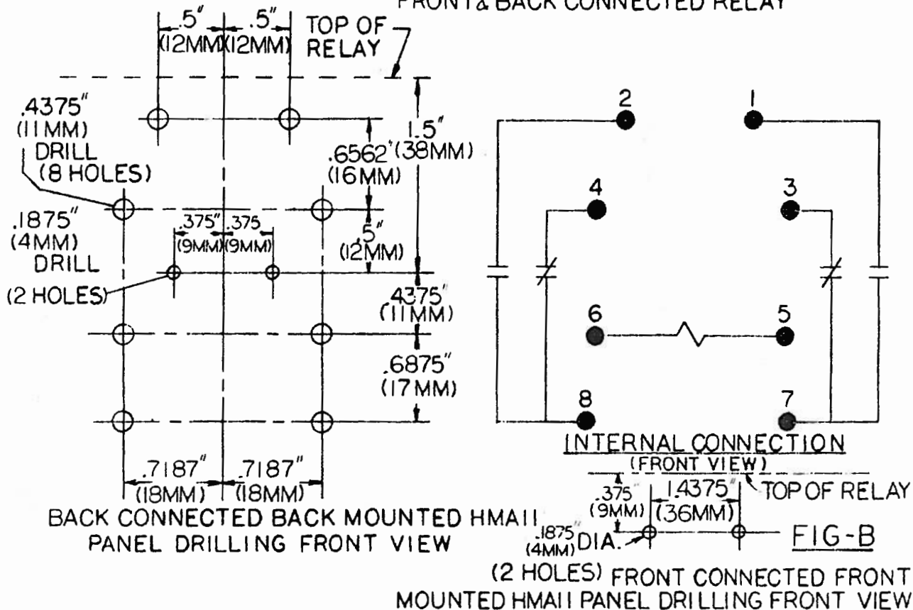
FIG. 2 (K-6400789 [8]); OUTLINE, PANEL DRILLING DIMENSIONS AND INTERNAL CONNECTIONS FOR TYPE HMA11A, HMA11B, HMA11E AND HMA11F RELAYS
