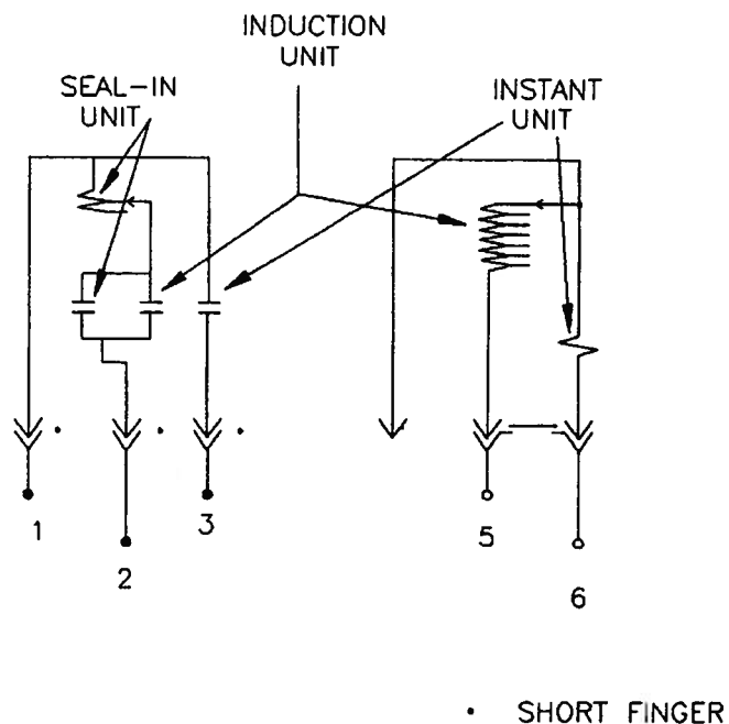
Fig. 12. (K-6209661 [11]) Internal Connections for the Type IAC51B Relay (Front View)
