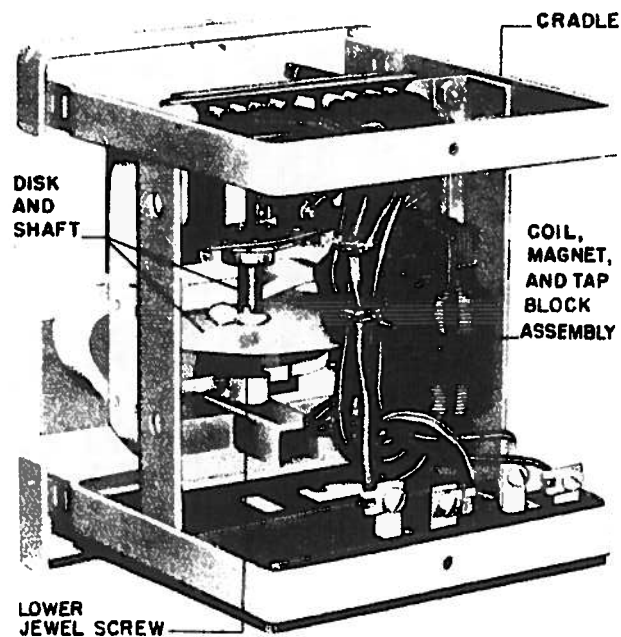
B - (8006997) Rear View
