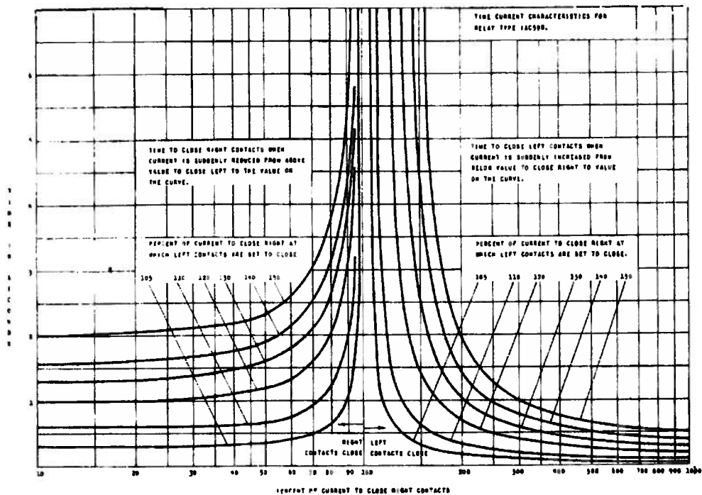
Figure 2. (K-6400289) Time-Current Characteristics for Type IAC59B Relay
