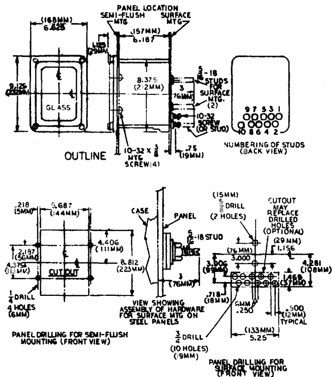
* Figure 6. (6209271-6) Outline and Panel Drilling for the Type IAC59A Relay
