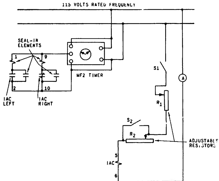
Figure 5. (K-6400302) Type IAC59A and IAC59B Relays, Test Connections
