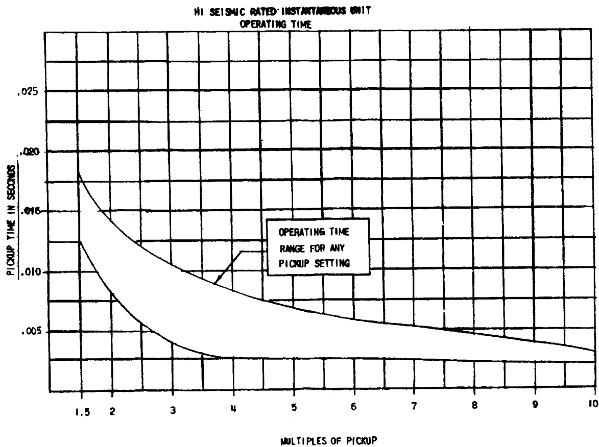
Fig. 19 (0208A8695 (1)) Time-Current Characteristics for the "Hi-G" Unit
