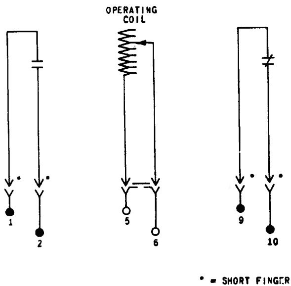
Figure 4. (K-6400432) Type IAC59C Relay Internal Connections (Front View).
