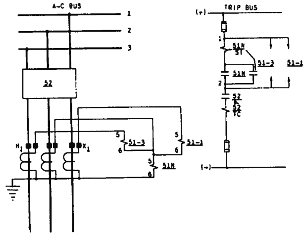
Fig. 4 (K-6375667-2) External Connections of Three Type IAC51A Relays used for Phase-to-Phase and Ground Overcurrent Portection of a 3-Phase Circuit.
