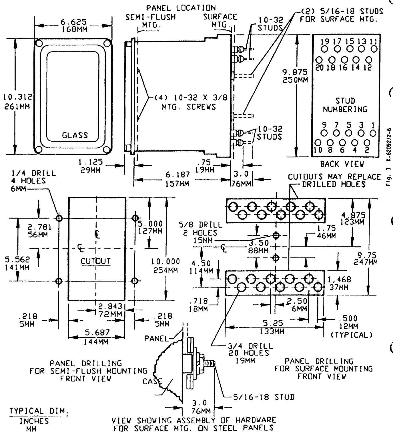
Fig. 3 Outline And Panel Drilling Dimensions For Type IAC51N Relay
