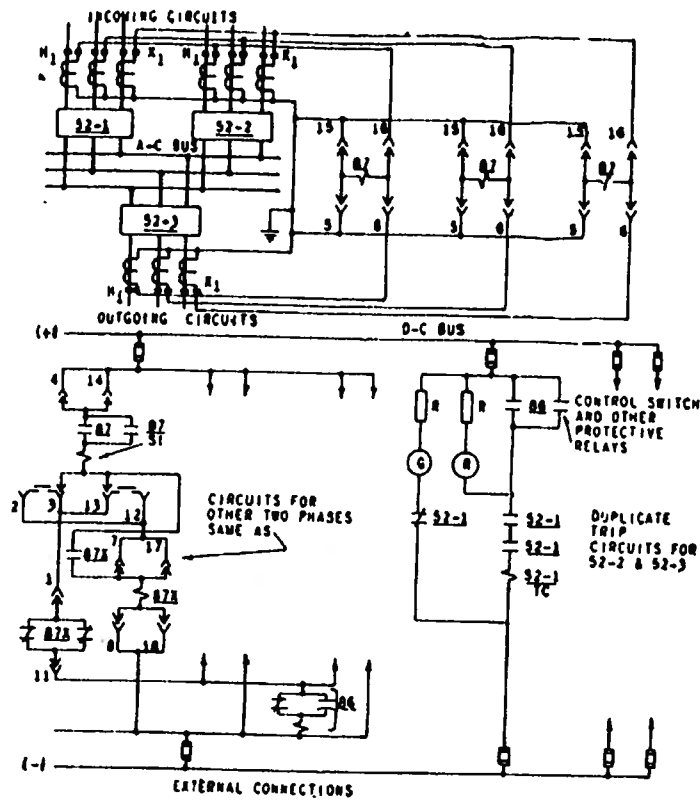
Fig. 1 Differential Protection Of A Bus Using Three Type IAC51M Relays
