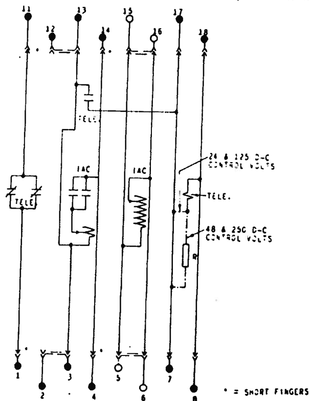
Fig. 2 Type IAC51M Relay, Internal Connections (Front View)
