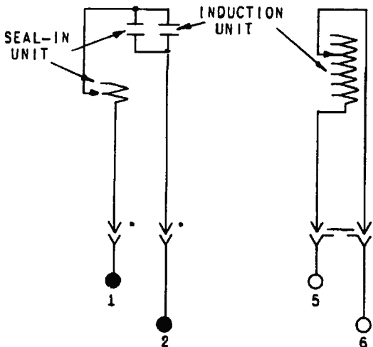
Fig. 11. (K-6209658-10) Internal Connections for the Type IAC51A Relay (Front View). *
