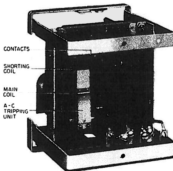
Fig. 5 Type IAC Relay with an A-C Trip Unit (Rear View)
