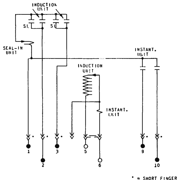
Fig. 17 Internal Connections for Type IAC54B
