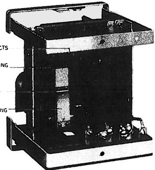
Fig. 5 Type IAC Relay with an A-C Trip Unit (Rear View)
