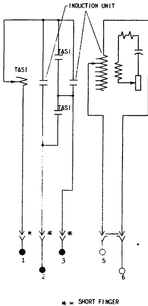
FIG. 12 (0165A7781-0) TYPE IAC78A RELAY INTERNAL CONNECTIONS (FRONT VIEW)
