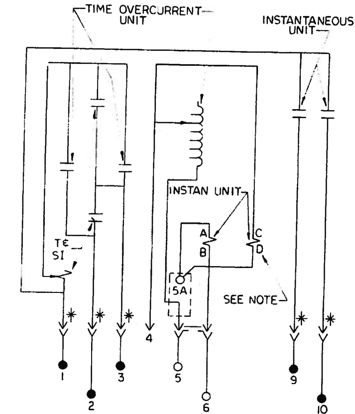
Figure 6 (K-6209662 [5]) Type IAC52A 800 Series Relay Internal Connections (Front View)
