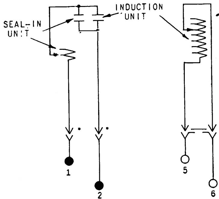
INTERNAL CONNECTIONS (FRONT VIEW) * = SHORT FINGER
