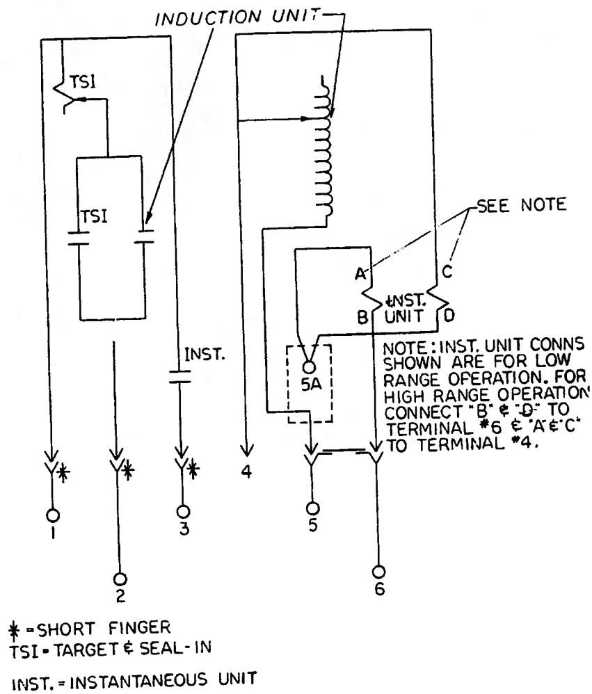
Figure 5 (0227A7196-1) Type IAC53B Internal Connections (Front View)
