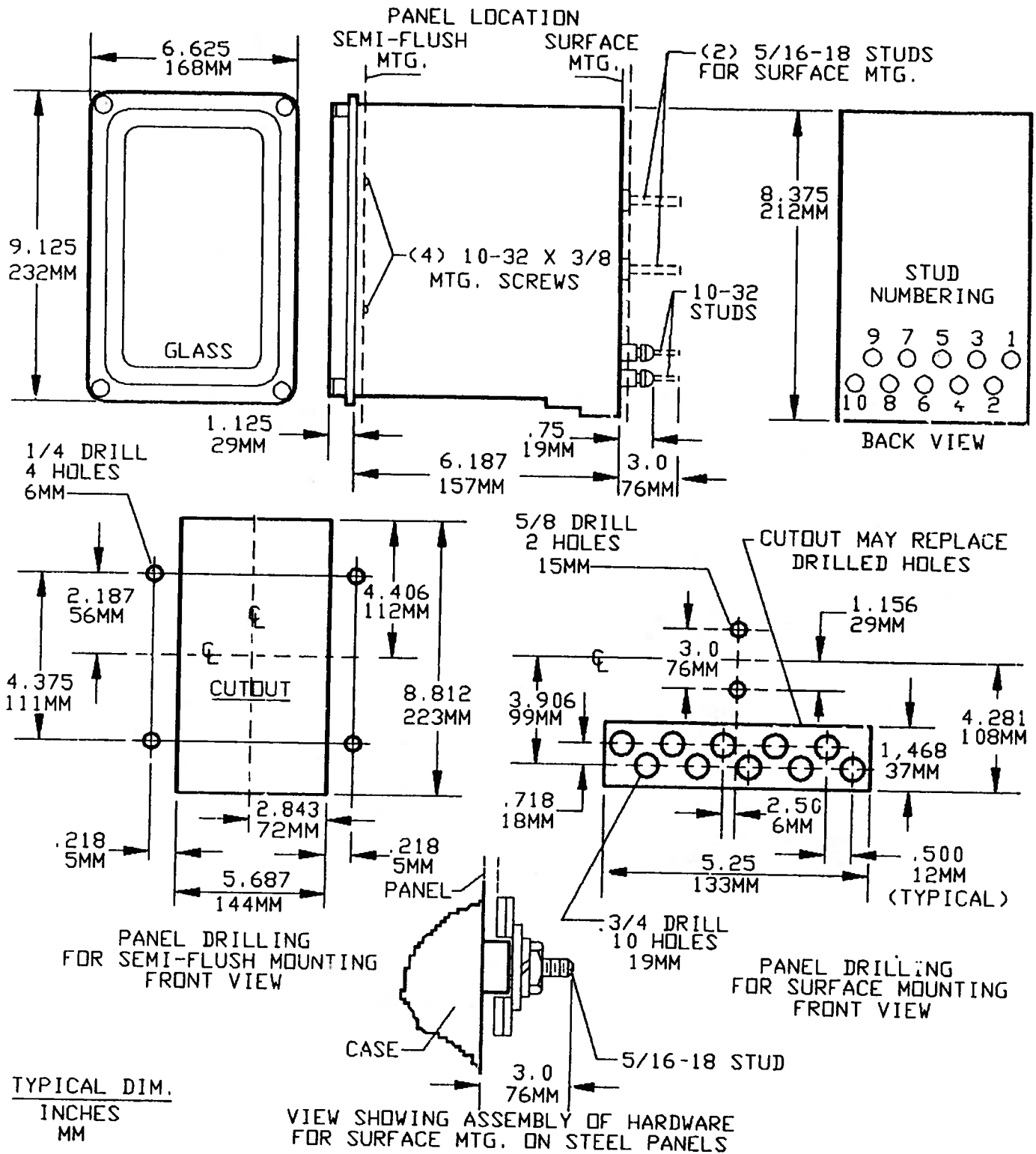
Figure 12 (6209271 [8]) Outline and Panel Drilling for IAC54B Relay
