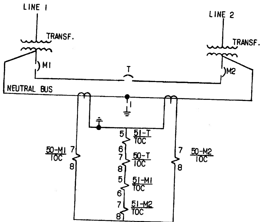
GROUND FAULT SCHEME FOR THE MAIN AND TIE BREAKERS OF A FOUR-WIRE DOUBLE ENDED LOAD CENTER WITH NEUTRAL GROUNDED AT ONE POINT.
