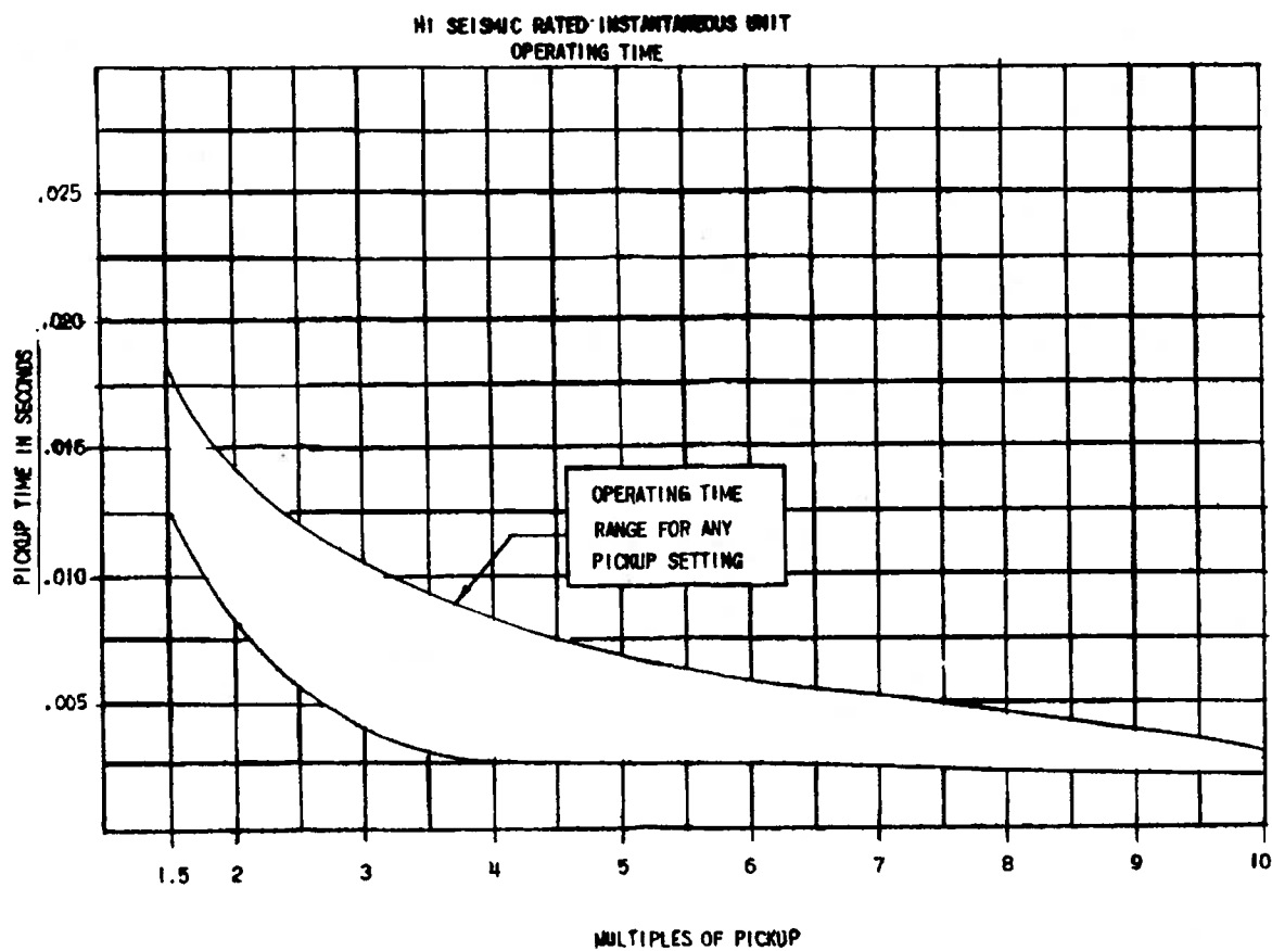
Fig. 19 (0208A8695 (1)) Time-Current Characteristics for the "Hi-C" Unit
