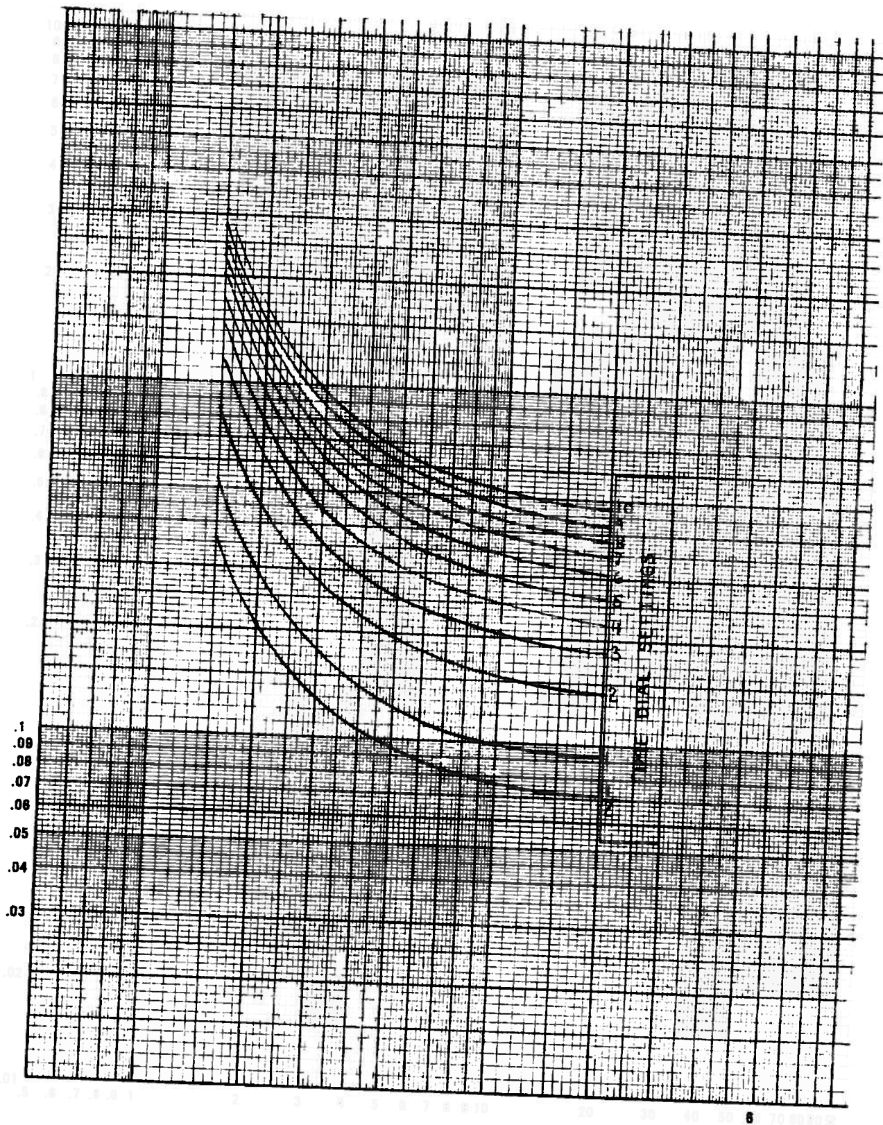
FIG. 1 (0183B4250-1) Time-Current Curves Of IAC95F(-)A Relay
