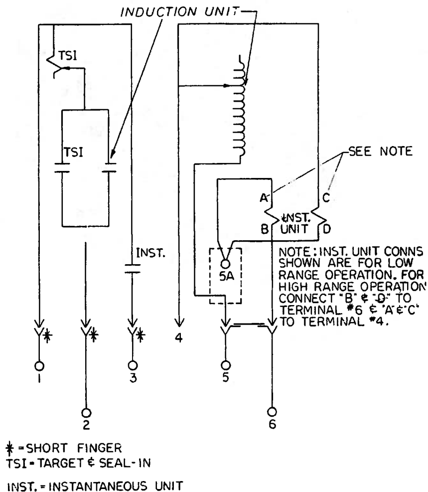
Figure 5 (0227A7196-1) Type IAC53B Internal Connections (Front View)
