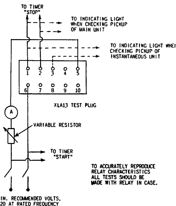
Fig. 16 (K-6154399-7) Testing Connections for Type IAC Relays such as Type IAC51A
