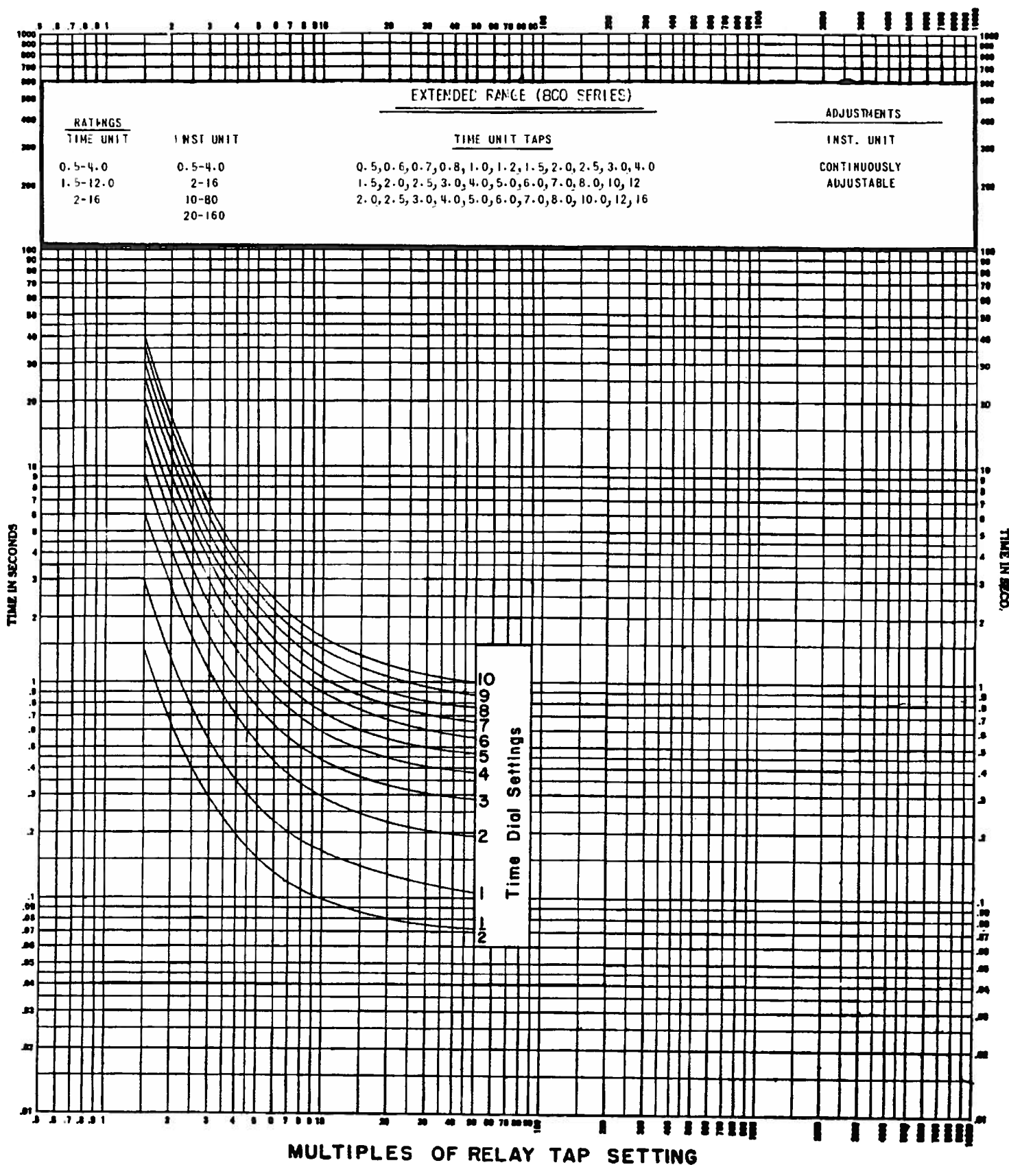
Fig. 7 (0888B0270-3) 60 Hertz Time-Current Characteristics for Relay-Type IAC80T
