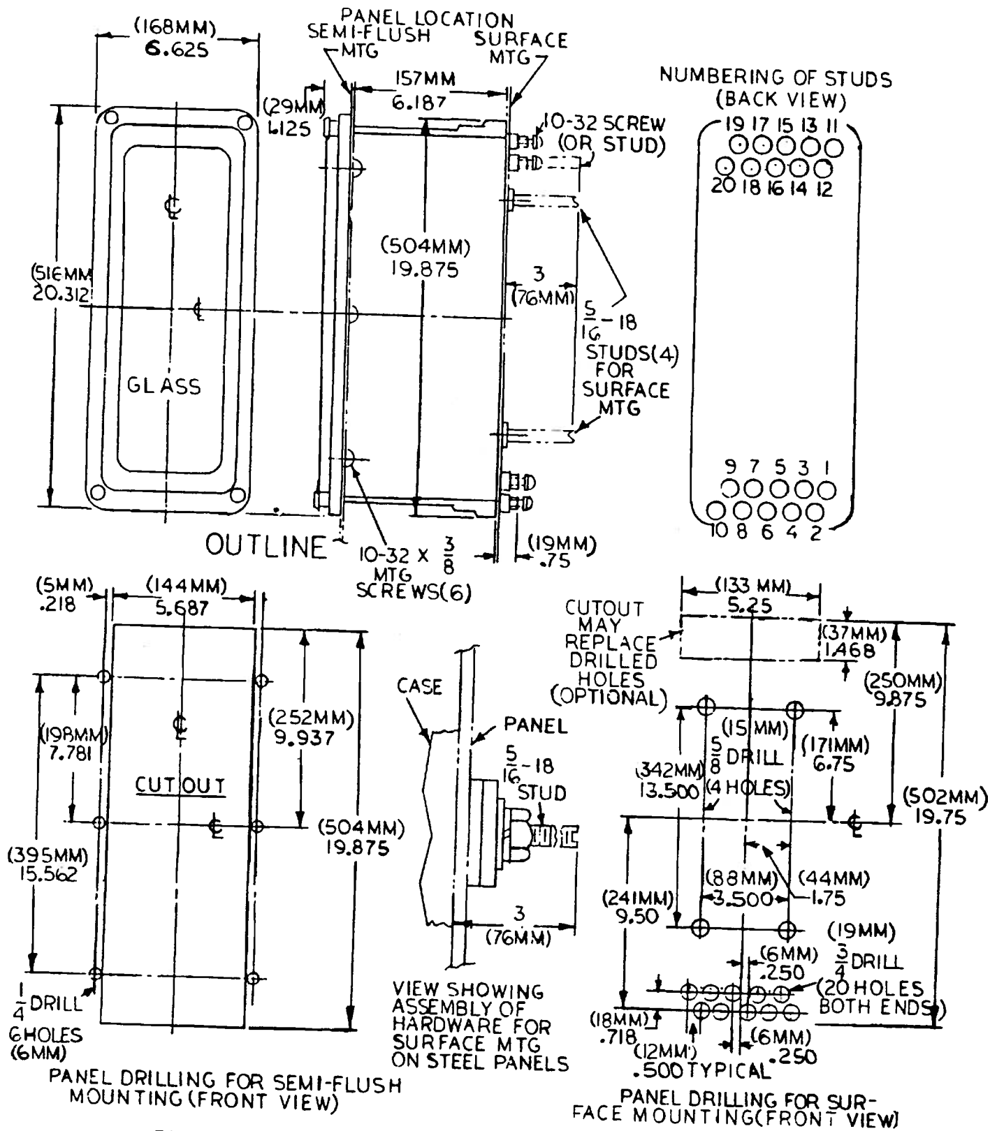
Fig. 15 (6209276-3) Outline and Panel Drilling Dimensions for the IAC60T, IAC80T and IAC90T Relays
