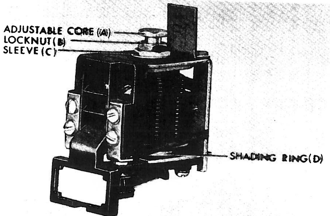
Figure 8 (8036365) Photograph: High Dropout Unit Construction
