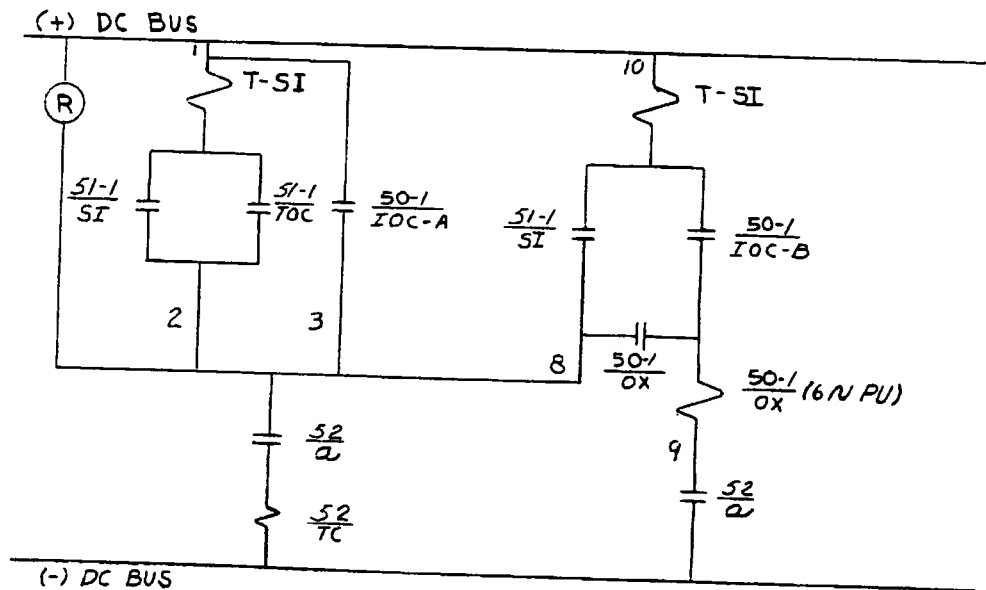
Figure 5 (0207A7826-0) External Connections Diagram for IAC66M Relay
