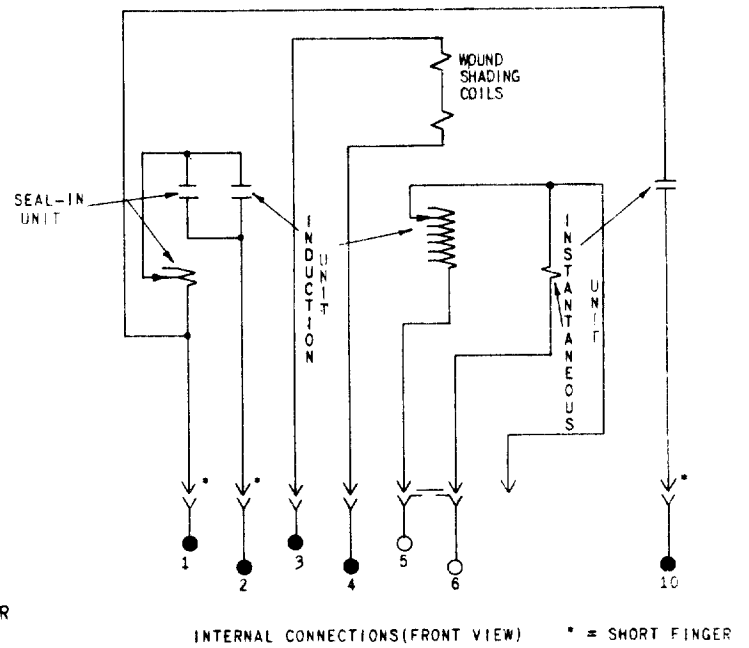
Fig. 4 (K-6400251-6) Internal Connections For Type IAC60B Relay (Front View)
