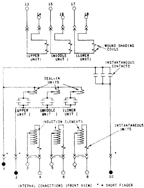
Fig. 5 (K-6400341-5) Internal Connections For Type IAC60J Relay (Front View)
