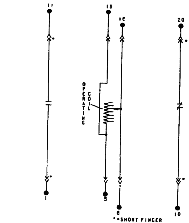
Figure 8 (K-6556476) Internal-Connection Diagram for Type-IAV53L and -IAV53N Relays
