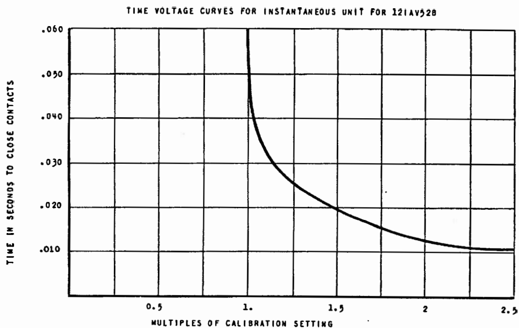
Fig. 2 (K-6507984) Time-Voltage Curve for Type IAV52B Relay
