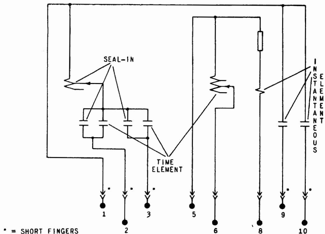
Fig. 1 (K-6375887) Internal Connections for Type IAV52B Relay (Front View)
