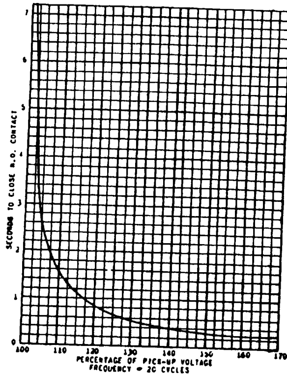
Figure 1 (362A645) Typical Voltage Time Curve
