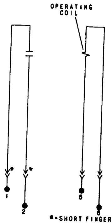
Figure 2 (362A535) Internal Connections for Type IAV51L Relay
