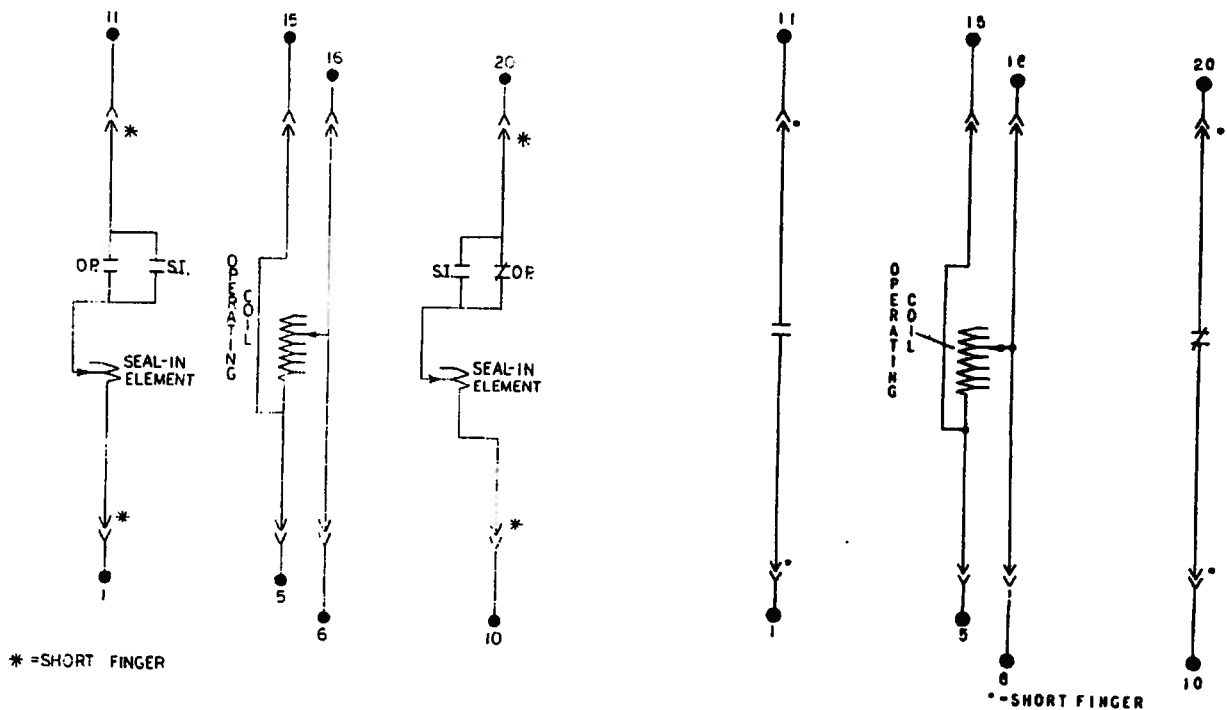
Figure 7 (K-6556475-1) Internal-Connection Diagram for Type-IAV53K Relay
