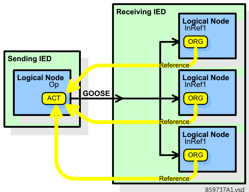
Figure 3-18: Logical nodes communicate with logical nodes
