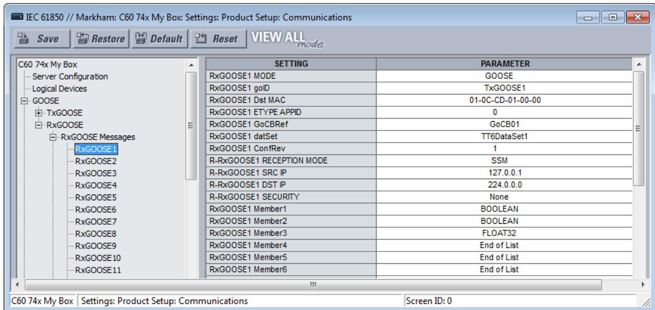
Figure 3-6: IEC 61850 RxGOOSE Messages panel
