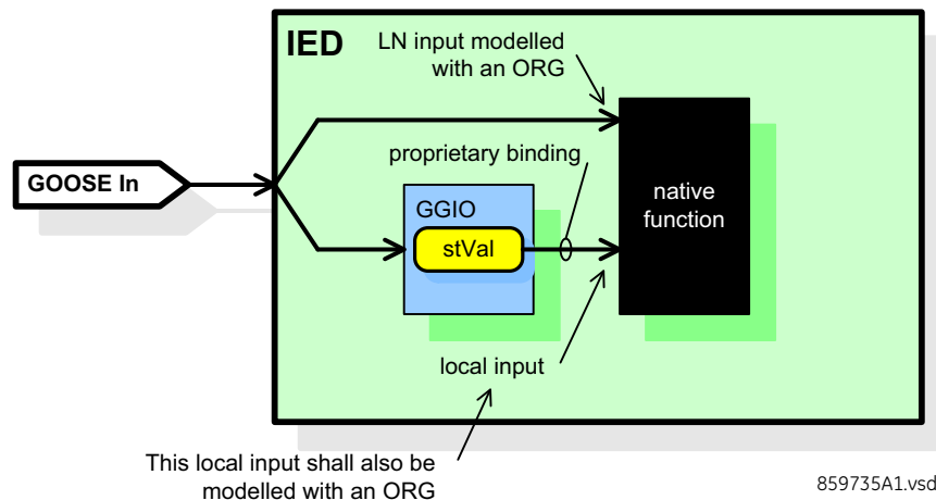
Figure 3-17: Mapping local inputs
