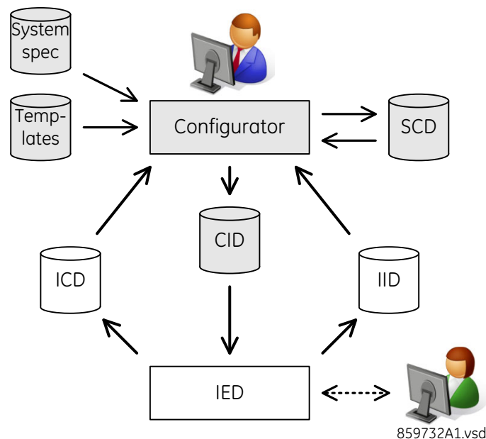
Figure 3-14: SCL file flow for IED configuration
