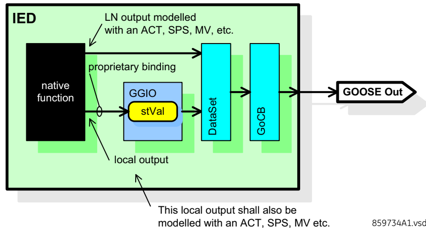
Figure 3-16: Mapping local outputs
