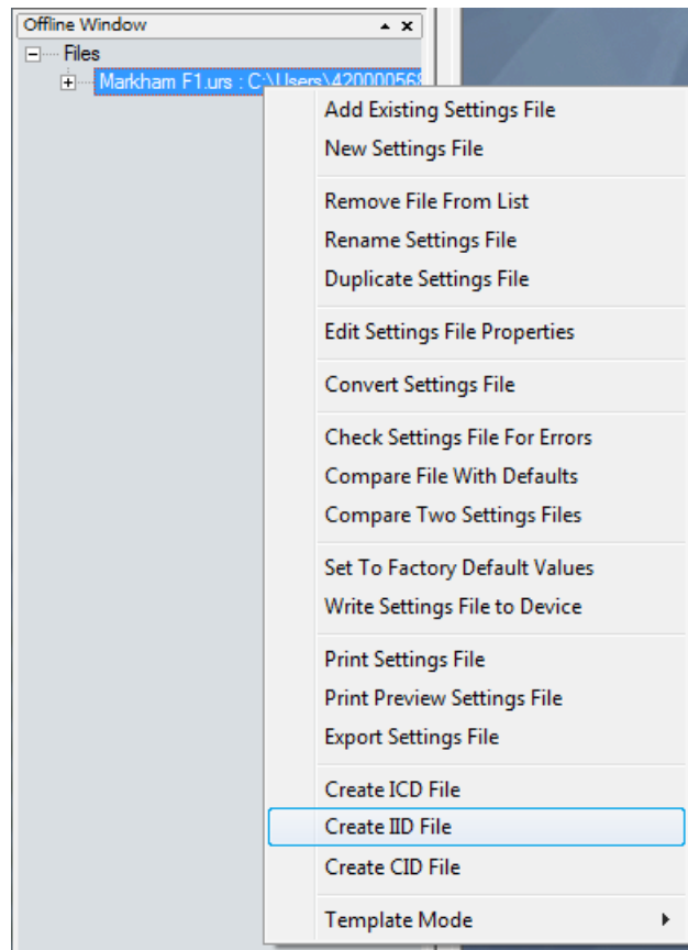
Figure 3-11: Creating CID file
