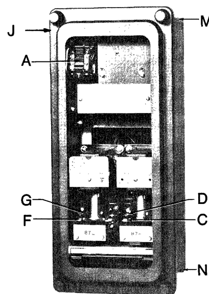
Fig. 1. Type PVD relay, front view
