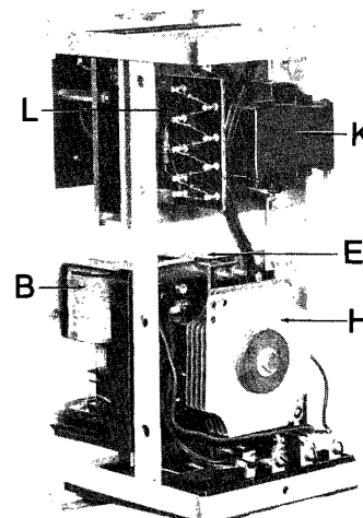
Fig. 2. Type PVD relay, rear view
